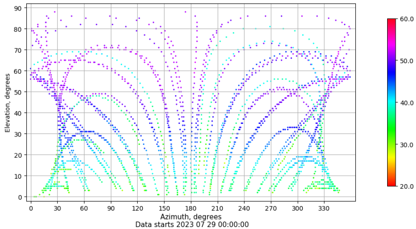
Azimuth-elevation plot for station VALC. Signal to Noise S1C Data file VALC00ESP_R_2023210.xtr
