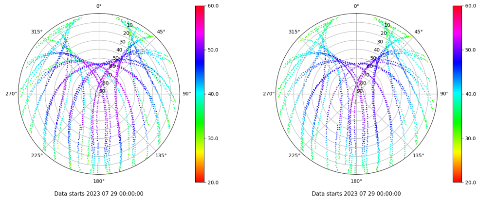
Skyplot for station VALC. Signal to Noise S1C Data file VALC00ESP_R_2023210.xtr Skyplot for station VALC. Signal to Noise S2C Data file VALC00ESP_R_2023210.xtr
