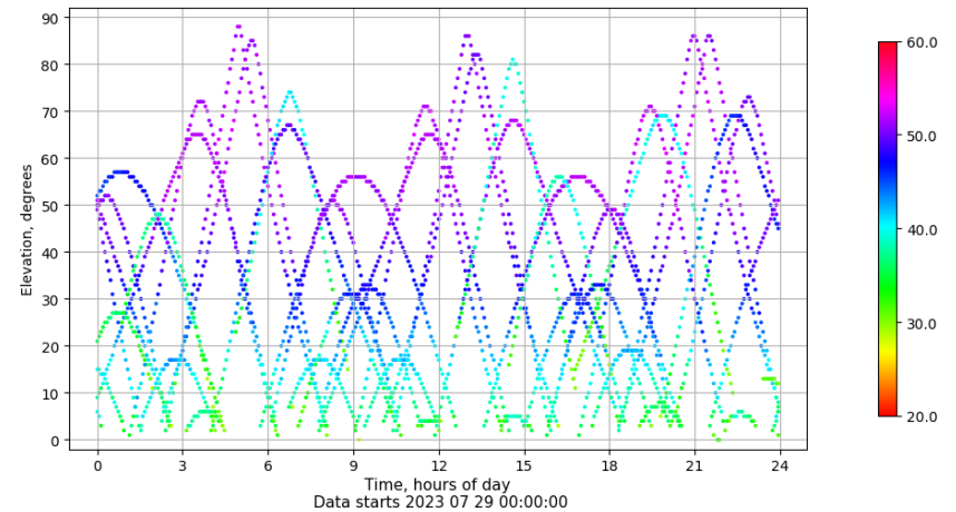
Time-elevation plot for station VALC. Signal to Noise S1C Data file VALC00ESP_R_2023210.xtr
