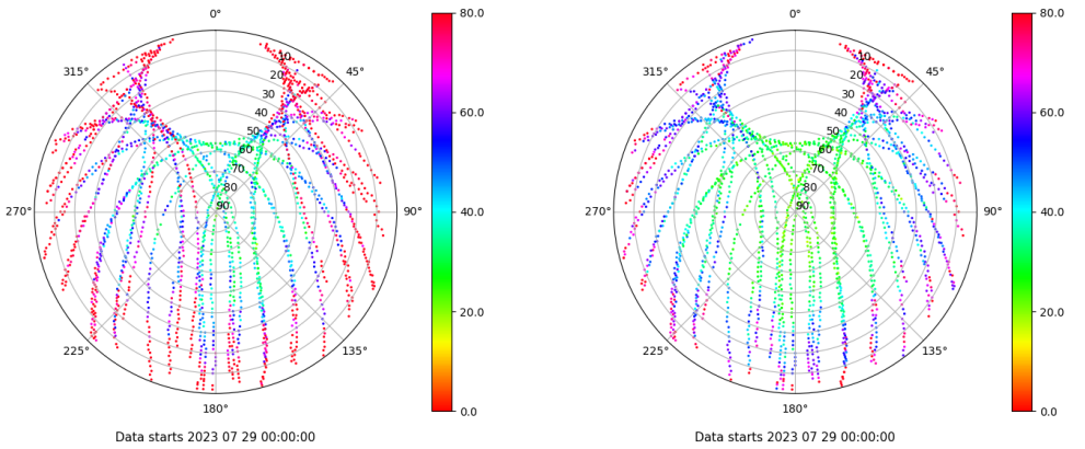
Skyplot for station VALC. Parameter M1C Data file VALC00ESP_R_2023210.xtr Skyplot for station VALC. Parameter M2C Data file VALC00ESP_R_2023210.xtr
