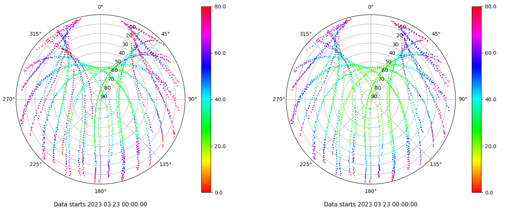
Skyplot for station VALC. Parameter M1C Data file VALC00ESP_R_2023082.xtr Skyplot for station VALC. Parameter M2C Data file VALC00ESP_R_2023082.xtr
