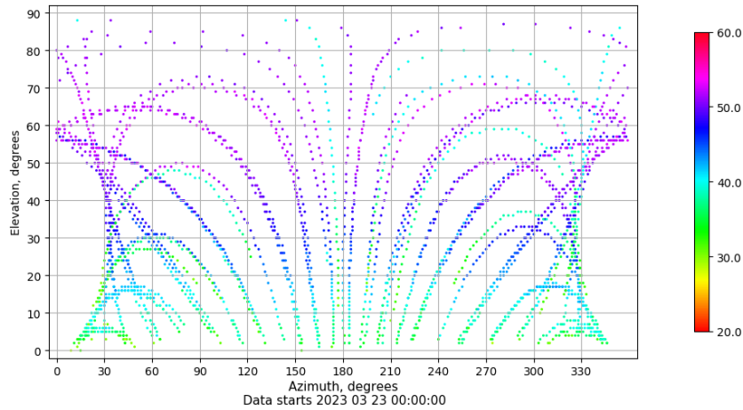
Azimuth-elevation plot for station VALC. Signal to Noise S1C Data file VALC00ESP_R_2023082.xtr
