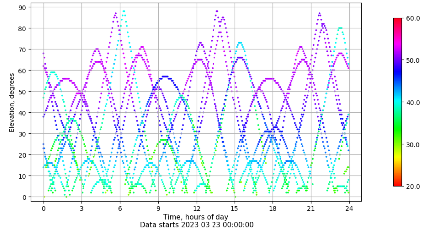
Time-elevation plot for station VALC. Signal to Noise S1C Data file VALC00ESP_R_2023082.xtr
