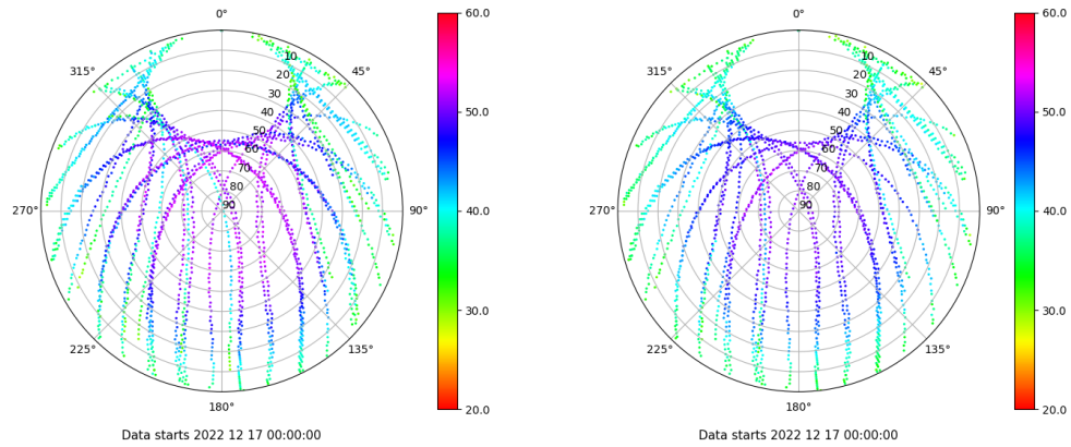
Skyplot for station VALC. Signal to Noise S1C Data file VALC00ESP_R_2022351.xtr Skyplot for station VALC. Signal to Noise S2C Data file VALC00ESP_R_2022351.xtr
