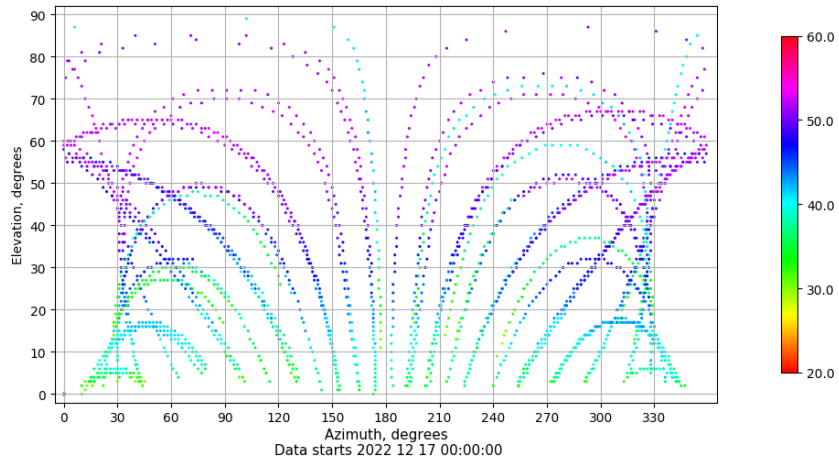
Azimuth-elevation plot for station VALC. Signal to Noise S1C Data file VALC00ESP_R_2022351.xtr
