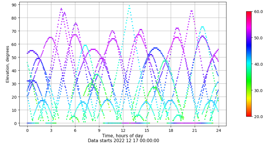
Time-elevation plot for station VALC. Signal to Noise S1C Data file VALC00ESP_R_2022351.xtr
