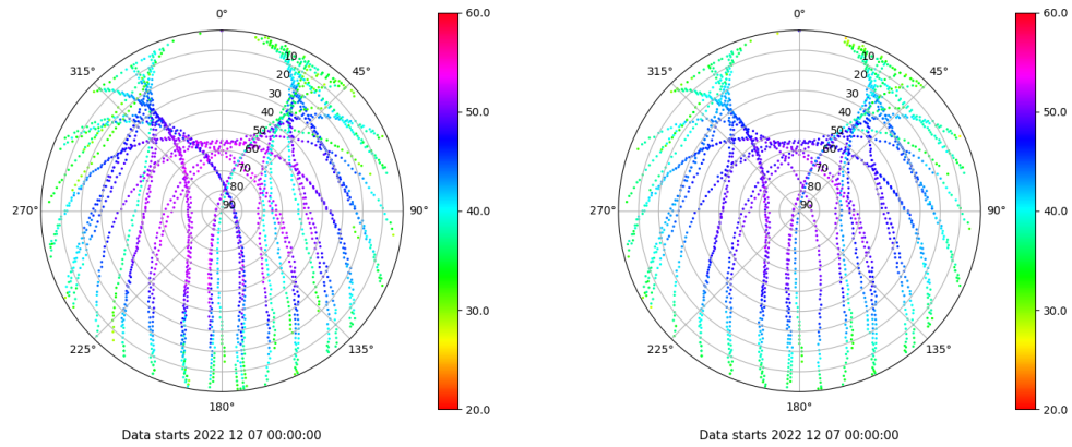
Skyplot for station VALC. Signal to Noise S1C Data file VALC00ESP_R_2022341.xtr Skyplot for station VALC. Signal to Noise S2C Data file VALC00ESP_R_2022341.xtr
