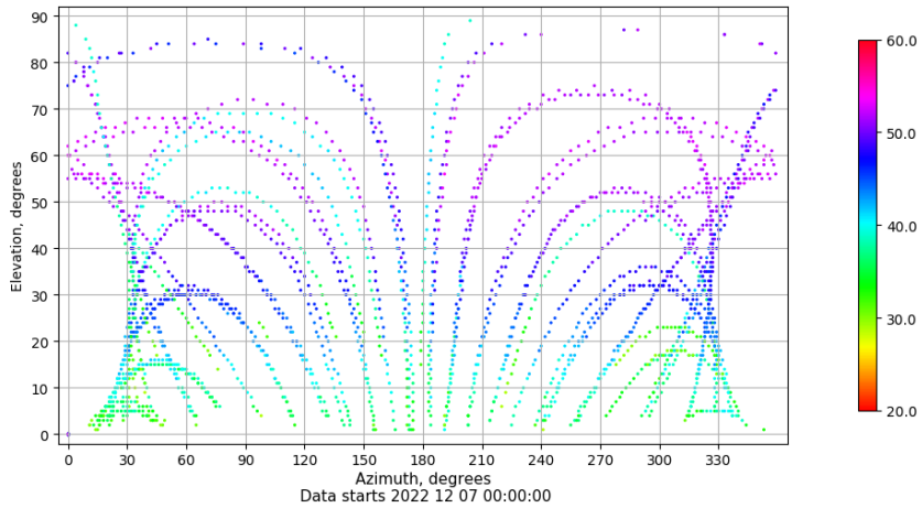
Azimuth-elevation plot for station VALC. Signal to Noise S1C Data file VALC00ESP_R_2022341.xtr
