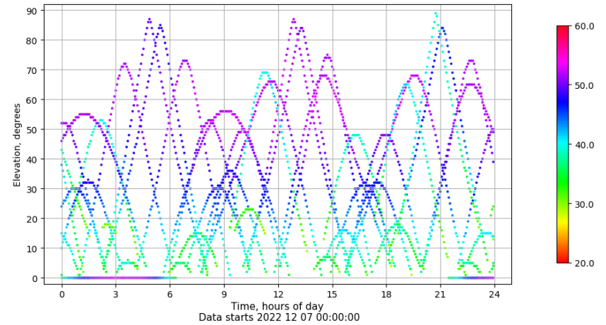
Time-elevation plot for station VALC. Signal to Noise S1C Data file VALC00ESP_R_2022341.xtr
