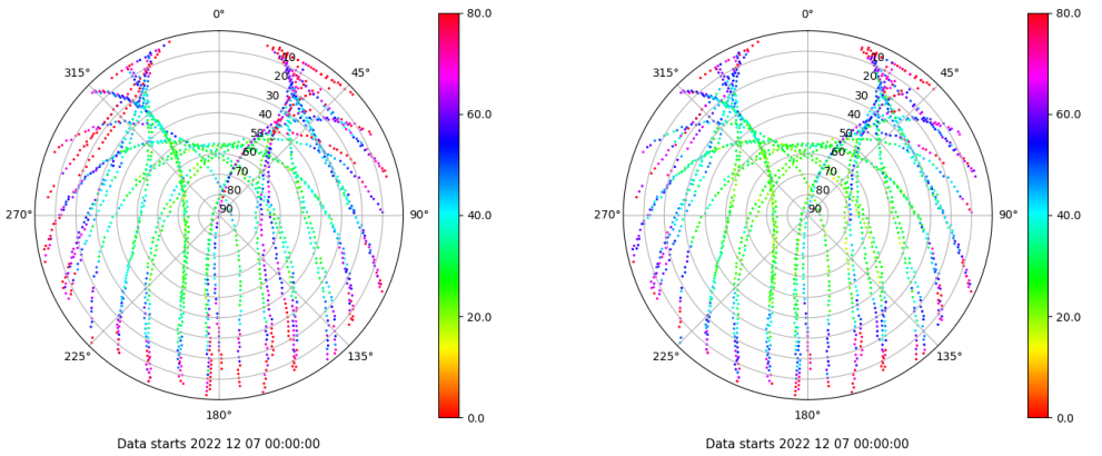
Skyplot for station VALC. Parameter M1C Data file VALC00ESP_R_2022341.xtr Skyplot for station VALC. Parameter M2C Data file VALC00ESP_R_2022341.xtr
