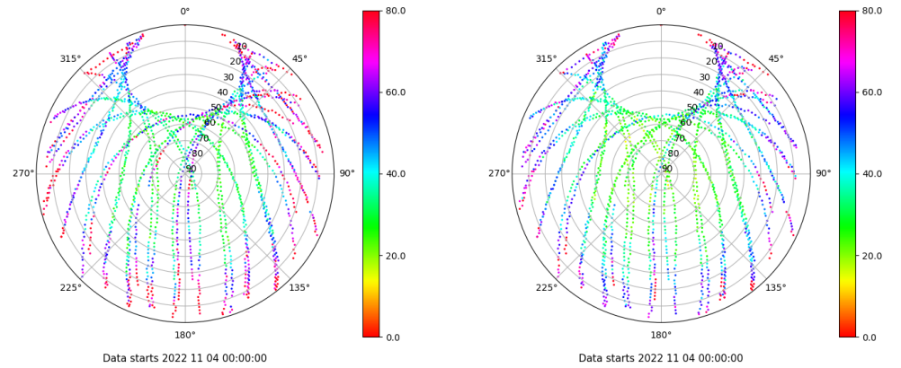
Skyplot for station VALC. Parameter M1C Data file VALC00ESP_R_2022308.xtr Skyplot for station VALC. Parameter M2C Data file VALC00ESP_R_2022308.xtr
