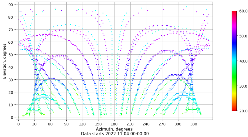
Azimuth-elevation plot for station VALC. Signal to Noise S1C Data file VALC00ESP_R_2022308.xtr
