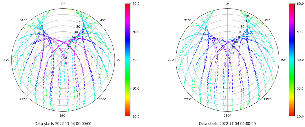
Skyplot for station VALC. Signal to Noise S1C Data file VALC00ESP_R_2022308.xtr Skyplot for station VALC. Signal to Noise S2C Data file VALC00ESP_R_2022308.xtr
