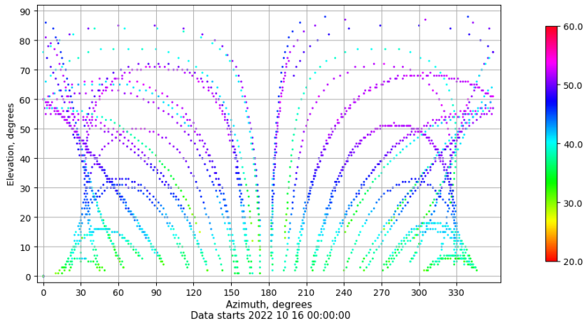
Azimuth-elevation plot for station VALC. Signal to Noise S1C Data file VALC00ESP_R_2022289.xtr
