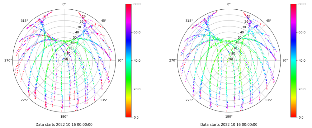
Skyplot for station VALC. Parameter M1C Data file VALC00ESP_R_2022289.xtr Skyplot for station VALC. Parameter M2C Data file VALC00ESP_R_2022289.xtr
