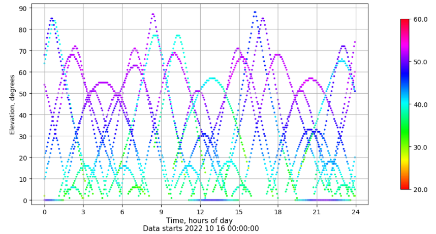
Time-elevation plot for station VALC. Signal to Noise S1C Data file VALC00ESP_R_2022289.xtr
