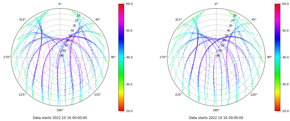
Skyplot for station VALC. Signal to Noise S1C Data file VALC00ESP_R_2022289.xtr Skyplot for station VALC. Signal to Noise S2C Data file VALC00ESP_R_2022289.xtr
