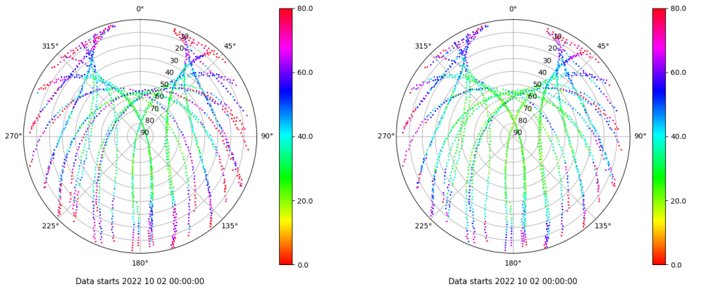
Skyplot for station VALC. Parameter M1C Data file VALC00ESP_R_2022275.xtr Skyplot for station VALC. Parameter M2C Data file VALC00ESP_R_2022275.xtr
