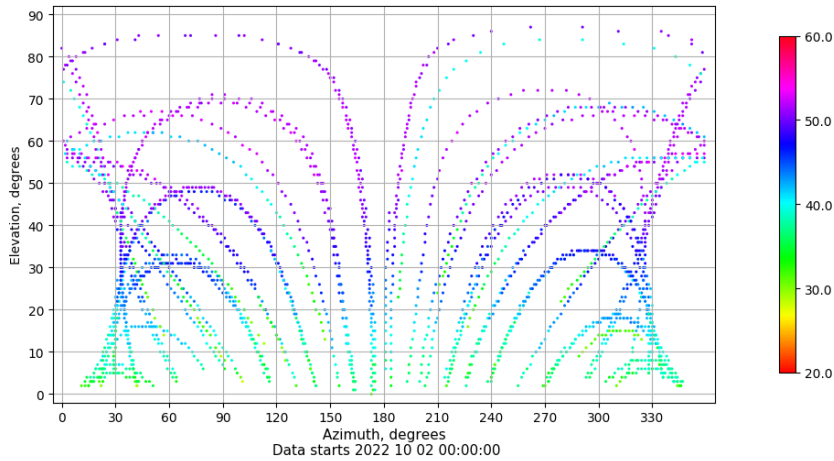
Azimuth-elevation plot for station VALC. Signal to Noise S1C Data file VALC00ESP_R_2022275.xtr
