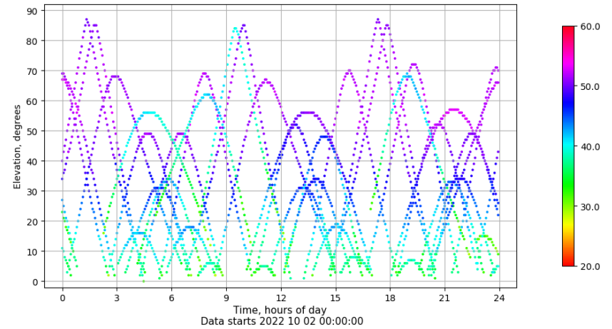
Time-elevation plot for station VALC. Signal to Noise S1C Data file VALC00ESP_R_2022275.xtr
