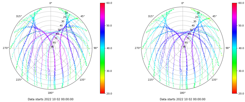
Skyplot for station VALC. Signal to Noise S1C Data file VALC00ESP_R_2022275.xtr Skyplot for station VALC. Signal to Noise S2C Data file VALC00ESP_R_2022275.xtr
