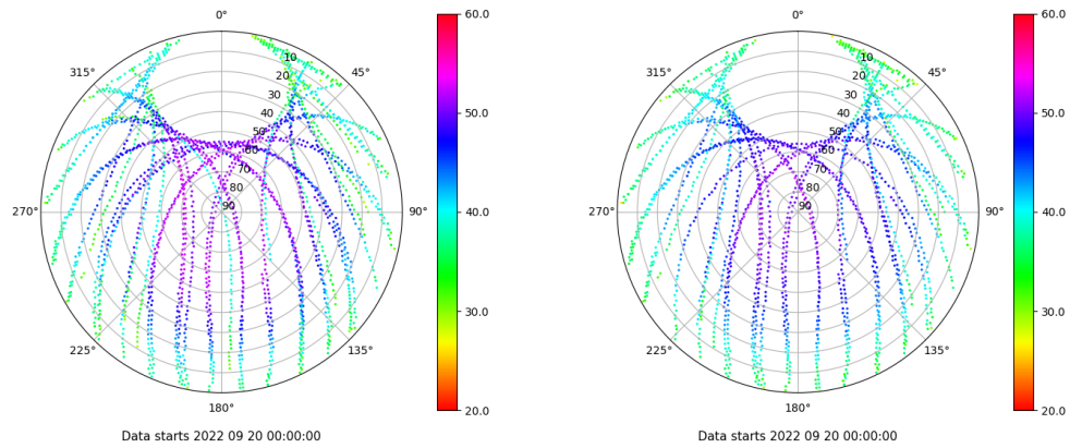
Skyplot for station VALC. Signal to Noise S1C Data file VALC00ESP_R_2022263.xtr Skyplot for station VALC. Signal to Noise S2C Data file VALC00ESP_R_2022263.xtr
