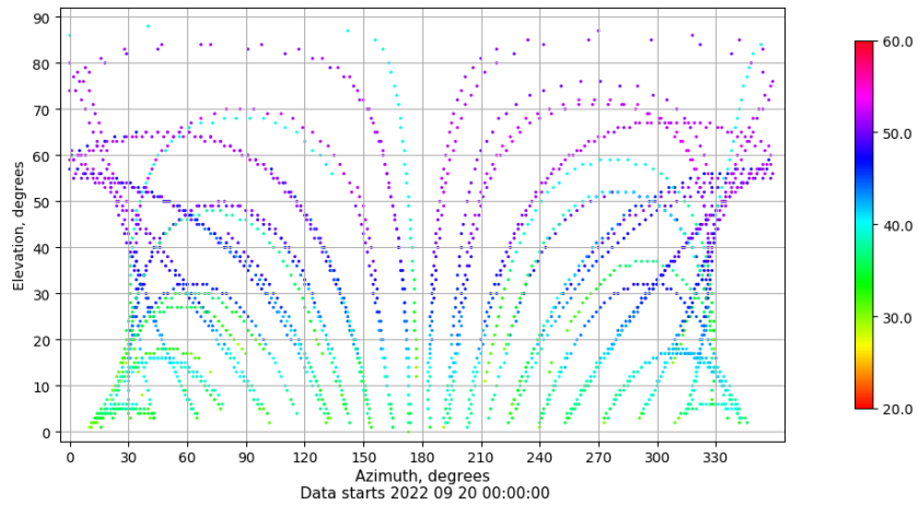
Azimuth-elevation plot for station VALC. Signal to Noise S1C Data file VALC00ESP_R_2022263.xtr
