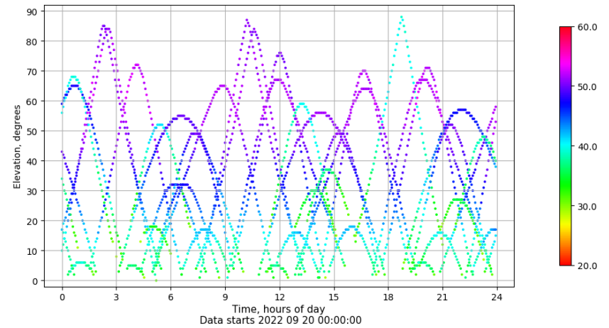
Time-elevation plot for station VALC. Signal to Noise S1C Data file VALC00ESP_R_2022263.xtr
