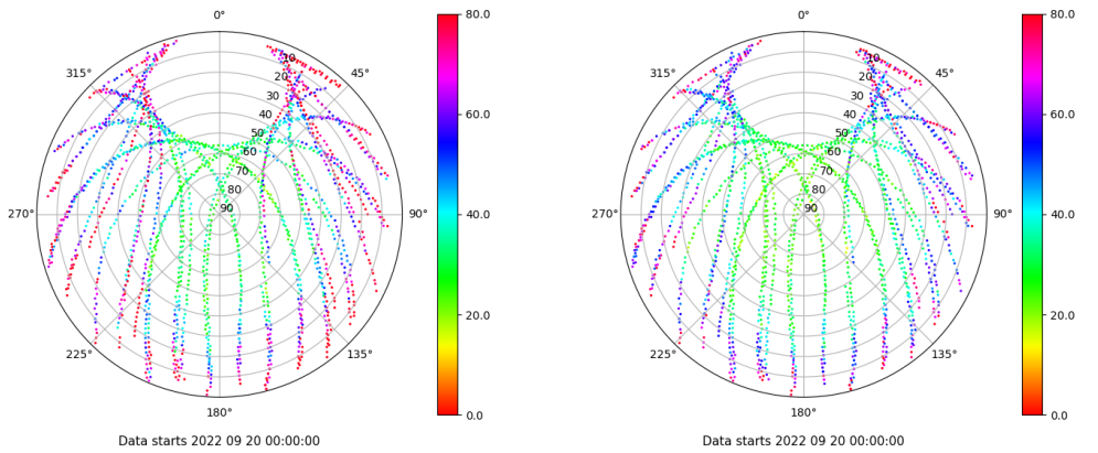
Skyplot for station VALC. Parameter M1C Data file VALC00ESP_R_2022263.xtr Skyplot for station VALC. Parameter M2C Data file VALC00ESP_R_2022263.xtr
