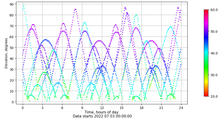
Time-elevation plot for station VALC. Signal to Noise S1C Data file VALC00ESP_R_2022184.xtr
