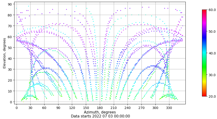
Azimuth-elevation plot for station VALC. Signal to Noise S1C Data file VALC00ESP_R_2022184.xtr
