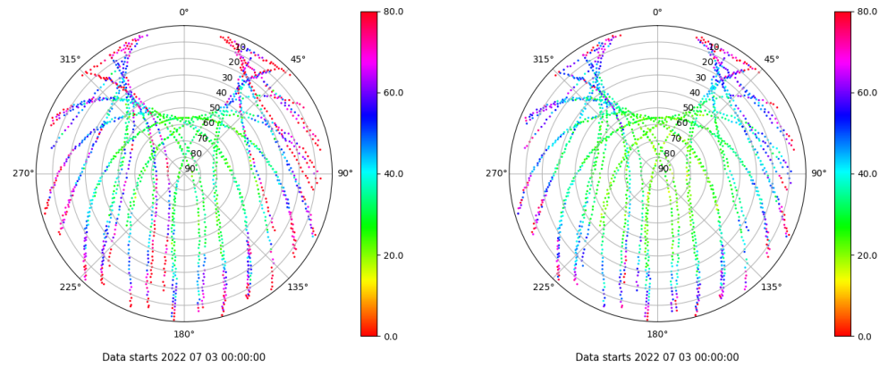
Skyplot for station VALC. Parameter M1C Data file VALC00ESP_R_2022184.xtr Skyplot for station VALC. Parameter M2C Data file VALC00ESP_R_2022184.xtr
