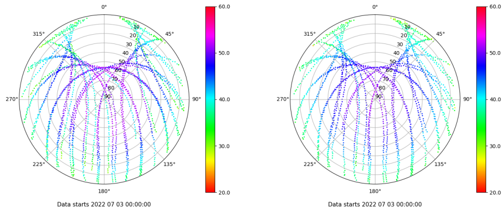
Skyplot for station VALC. Signal to Noise S1C Data file VALC00ESP_R_2022184.xtr Skyplot for station VALC. Signal to Noise S2C Data file VALC00ESP_R_2022184.xtr
