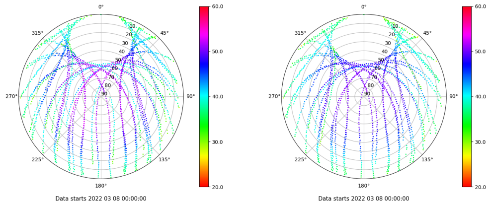
Skyplot for station VALC. Signal to Noise S1C Data file VALC00ESP_R_2022067.xtr Skyplot for station VALC. Signal to Noise S2C Data file VALC00ESP_R_2022067.xtr
