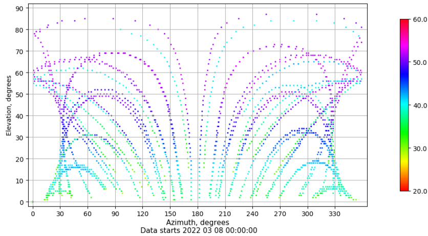
Azimuth-elevation plot for station VALC. Signal to Noise S1C Data file VALC00ESP_R_2022067.xtr
