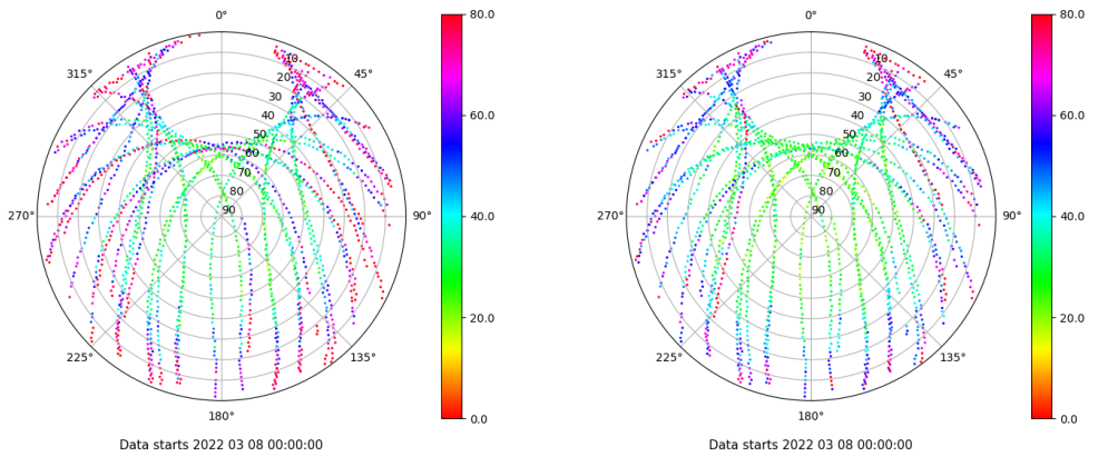
Skyplot for station VALC. Parameter M1C Data file VALC00ESP_R_2022067.xtr Skyplot for station VALC. Parameter M2C Data file VALC00ESP_R_2022067.xtr
