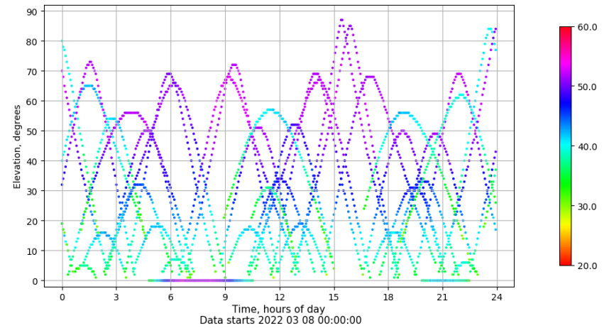
Time-elevation plot for station VALC. Signal to Noise S1C Data file VALC00ESP_R_2022067.xtr
