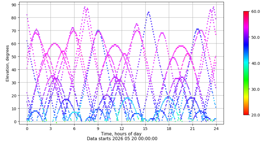
Time-elevation plot for station VALA. Signal to Noise S1C Data file VALA00ESP_R_2026140.xtr
