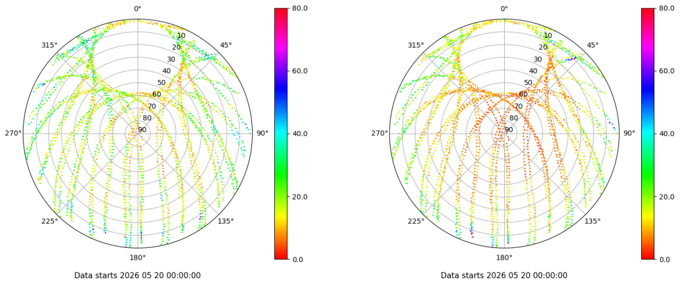
Skyplot for station VALA. Parameter M1C Data file VALA00ESP_R_2026140.xtr Skyplot for station VALA. Parameter M2C Data file VALA00ESP_R_2026140.xtr
