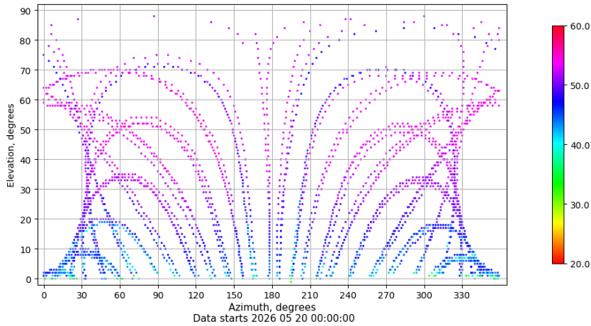
Azimuth-elevation plot for station VALA. Signal to Noise S1C Data file VALA00ESP_R_2026140.xtr
