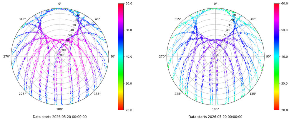
Skyplot for station VALA. Signal to Noise S1C Data file VALA00ESP_R_2026140.xtr Skyplot for station VALA. Signal to Noise S2C Data file VALA00ESP_R_2026140.xtr
