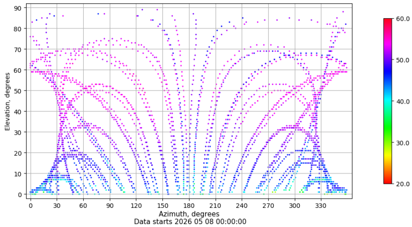
Azimuth-elevation plot for station VALA. Signal to Noise S1C Data file VALA00ESP_R_2026128.xtr
