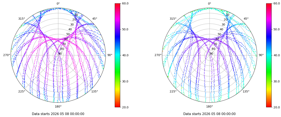
Skyplot for station VALA. Signal to Noise S1C Data file VALA00ESP_R_2026128.xtr Skyplot for station VALA. Signal to Noise S2C Data file VALA00ESP_R_2026128.xtr
