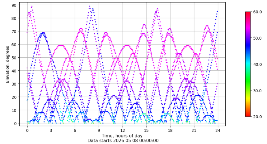
Time-elevation plot for station VALA. Signal to Noise S1C Data file VALA00ESP_R_2026128.xtr
