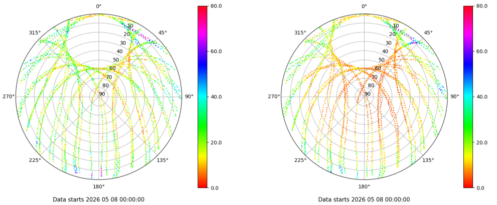
Skyplot for station VALA. Parameter M1C Data file VALA00ESP_R_2026128.xtr Skyplot for station VALA. Parameter M2C Data file VALA00ESP_R_2026128.xtr
