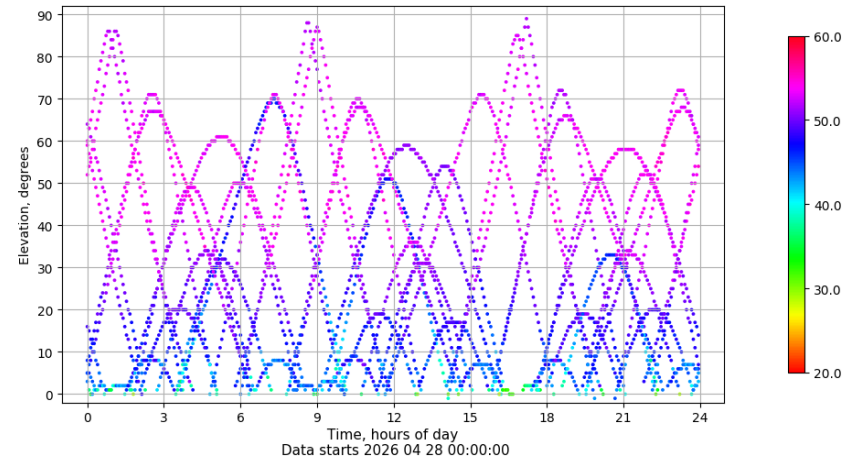
Time-elevation plot for station VALA. Signal to Noise S1C Data file VALA00ESP_R_2026118.xtr
