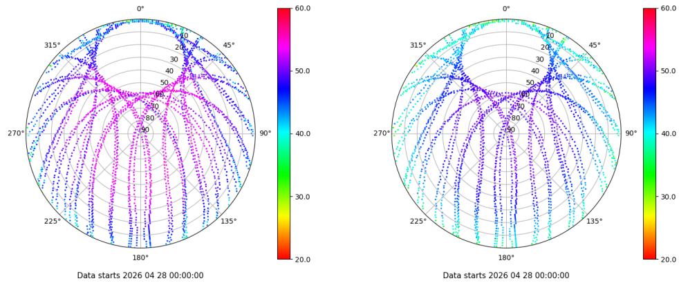
Skyplot for station VALA. Signal to Noise S1C Data file VALA00ESP_R_2026118.xtr Skyplot for station VALA. Signal to Noise S2C Data file VALA00ESP_R_2026118.xtr
