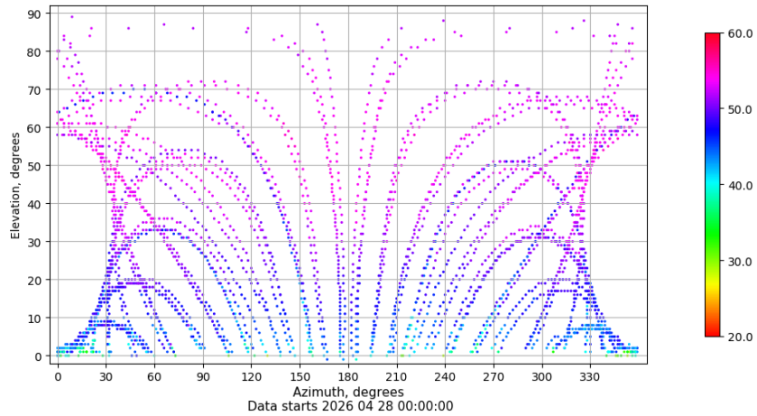
Azimuth-elevation plot for station VALA. Signal to Noise S1C Data file VALA00ESP_R_2026118.xtr
