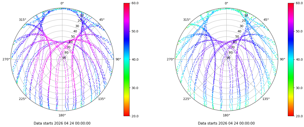
Skyplot for station VALA. Signal to Noise S1C Data file VALA00ESP_R_2026114.xtr Skyplot for station VALA. Signal to Noise S2C Data file VALA00ESP_R_2026114.xtr
