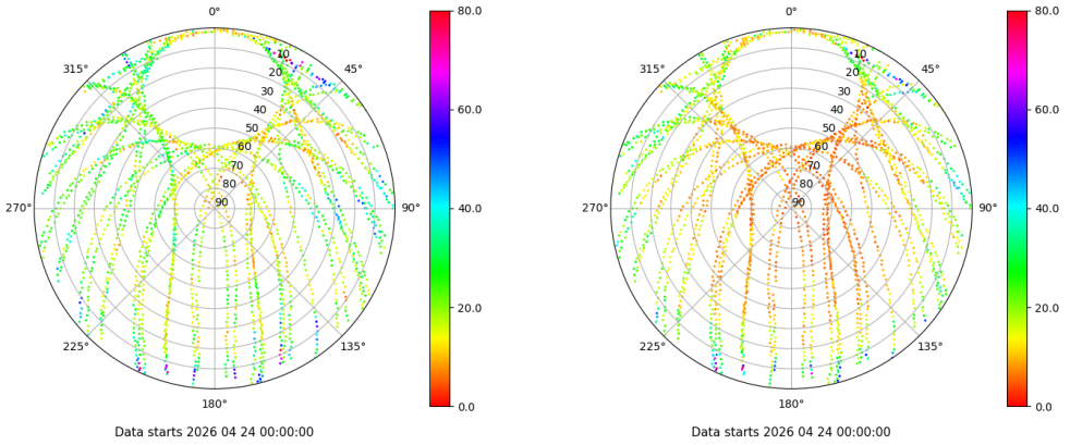
Skyplot for station VALA. Parameter M1C Data file VALA00ESP_R_2026114.xtr Skyplot for station VALA. Parameter M2C Data file VALA00ESP_R_2026114.xtr
