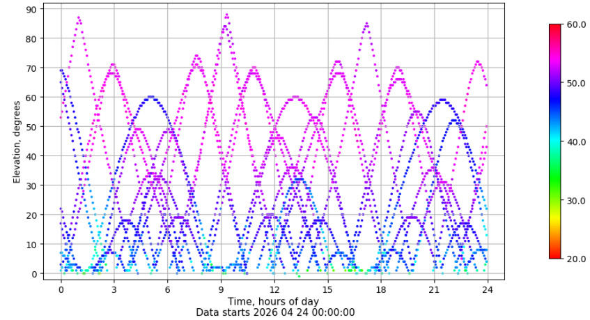
Time-elevation plot for station VALA. Signal to Noise S1C Data file VALA00ESP_R_2026114.xtr
