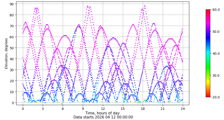
Time-elevation plot for station VALA. Signal to Noise S1C Data file VALA00ESP_R_2026102.xtr
