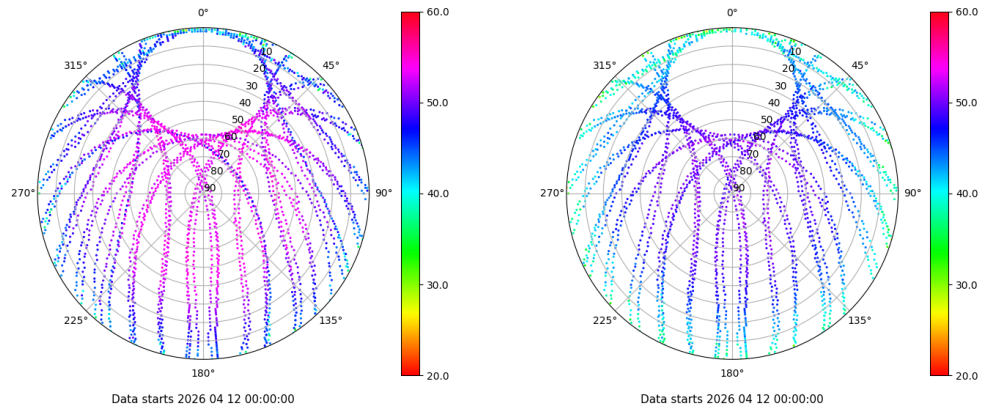
Skyplot for station VALA. Signal to Noise S1C Data file VALA00ESP_R_2026102.xtr Skyplot for station VALA. Signal to Noise S2C Data file VALA00ESP_R_2026102.xtr
