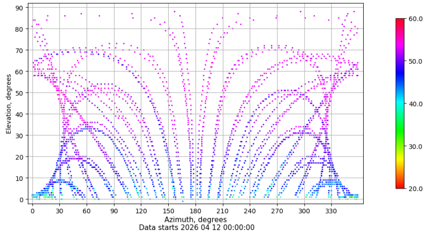
Azimuth-elevation plot for station VALA. Signal to Noise S1C Data file VALA00ESP_R_2026102.xtr
