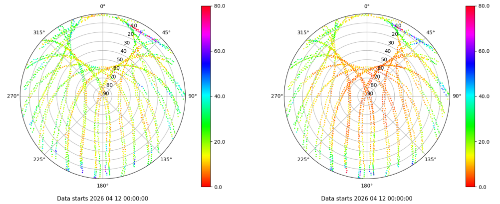
Skyplot for station VALA. Parameter M1C Data file VALA00ESP_R_2026102.xtr Skyplot for station VALA. Parameter M2C Data file VALA00ESP_R_2026102.xtr
