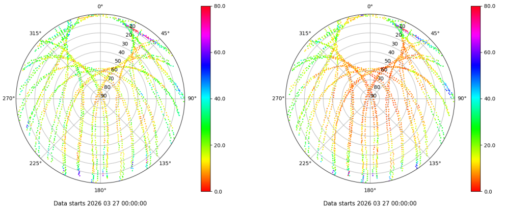
Skyplot for station VALA. Parameter M1C Data file VALA00ESP_R_2026086.xtr Skyplot for station VALA. Parameter M2C Data file VALA00ESP_R_2026086.xtr
