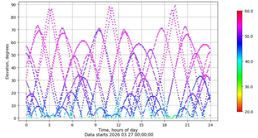
Time-elevation plot for station VALA. Signal to Noise S1C Data file VALA00ESP_R_2026086.xtr
