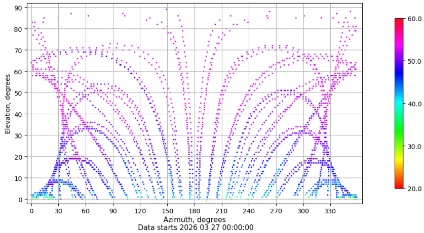
Azimuth-elevation plot for station VALA. Signal to Noise S1C Data file VALA00ESP_R_2026086.xtr
