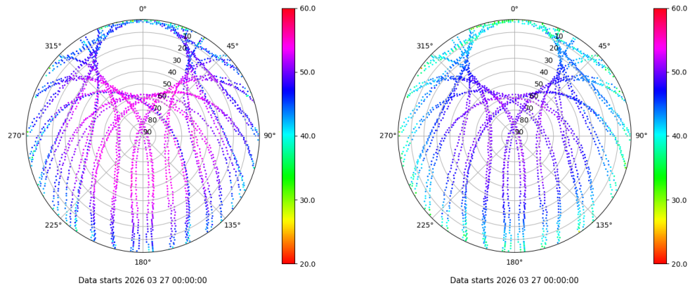
Skyplot for station VALA. Signal to Noise S1C Data file VALA00ESP_R_2026086.xtr Skyplot for station VALA. Signal to Noise S2C Data file VALA00ESP_R_2026086.xtr
