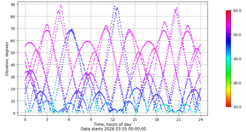
Time-elevation plot for station VALA. Signal to Noise S1C Data file VALA00ESP_R_2026064.xtr
