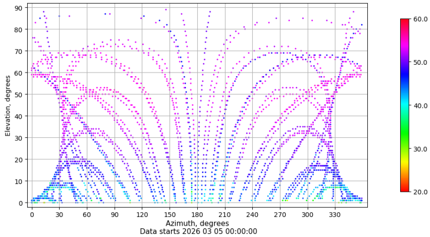
Azimuth-elevation plot for station VALA. Signal to Noise S1C Data file VALA00ESP_R_2026064.xtr
