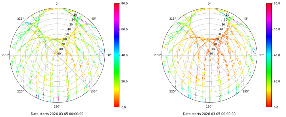
Skyplot for station VALA. Parameter M1C Data file VALA00ESP_R_2026064.xtr Skyplot for station VALA. Parameter M2C Data file VALA00ESP_R_2026064.xtr
