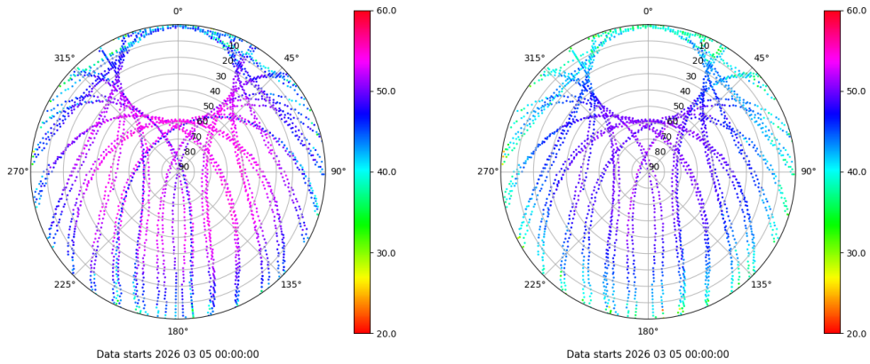
Skyplot for station VALA. Signal to Noise S1C Data file VALA00ESP_R_2026064.xtr Skyplot for station VALA. Signal to Noise S2C Data file VALA00ESP_R_2026064.xtr
