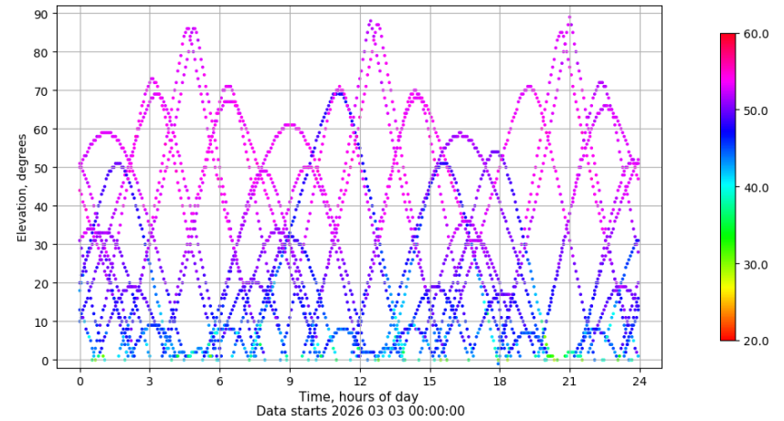
Time-elevation plot for station VALA. Signal to Noise S1C Data file VALA00ESP_R_2026062.xtr
