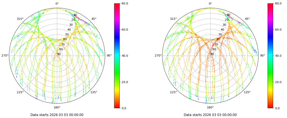
Skyplot for station VALA. Parameter M1C Data file VALA00ESP_R_2026062.xtr Skyplot for station VALA. Parameter M2C Data file VALA00ESP_R_2026062.xtr
