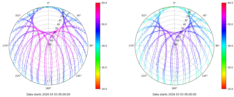
Skyplot for station VALA. Signal to Noise S1C Data file VALA00ESP_R_2026062.xtr Skyplot for station VALA. Signal to Noise S2C Data file VALA00ESP_R_2026062.xtr
