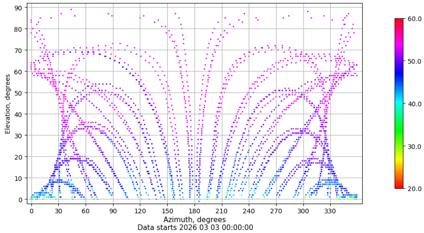
Azimuth-elevation plot for station VALA. Signal to Noise S1C Data file VALA00ESP_R_2026062.xtr
