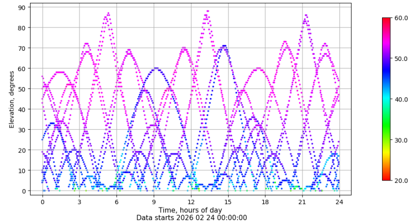
Time-elevation plot for station VALA. Signal to Noise S1C Data file VALA00ESP_R_2026055.xtr
