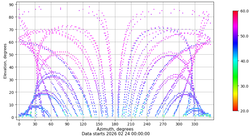
Azimuth-elevation plot for station VALA. Signal to Noise S1C Data file VALA00ESP_R_2026055.xtr
