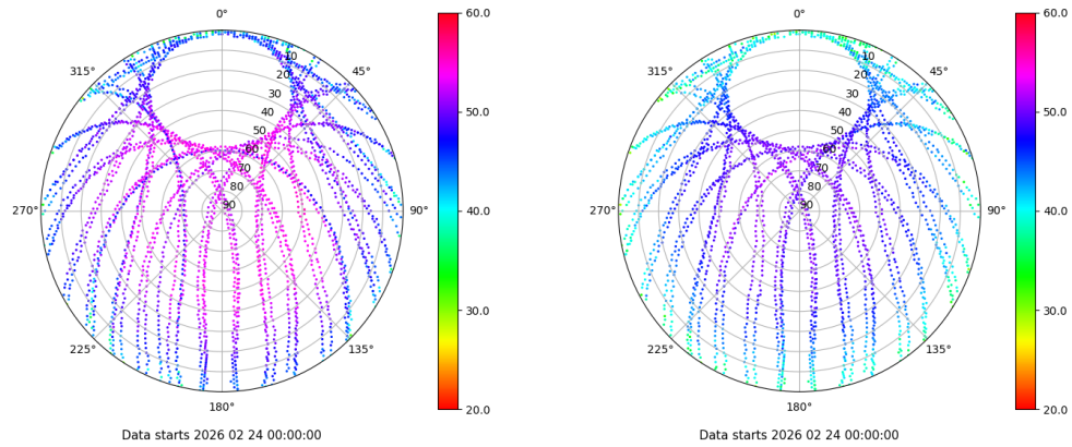
Skyplot for station VALA. Signal to Noise S1C Data file VALA00ESP_R_2026055.xtr Skyplot for station VALA. Signal to Noise S2C Data file VALA00ESP_R_2026055.xtr
