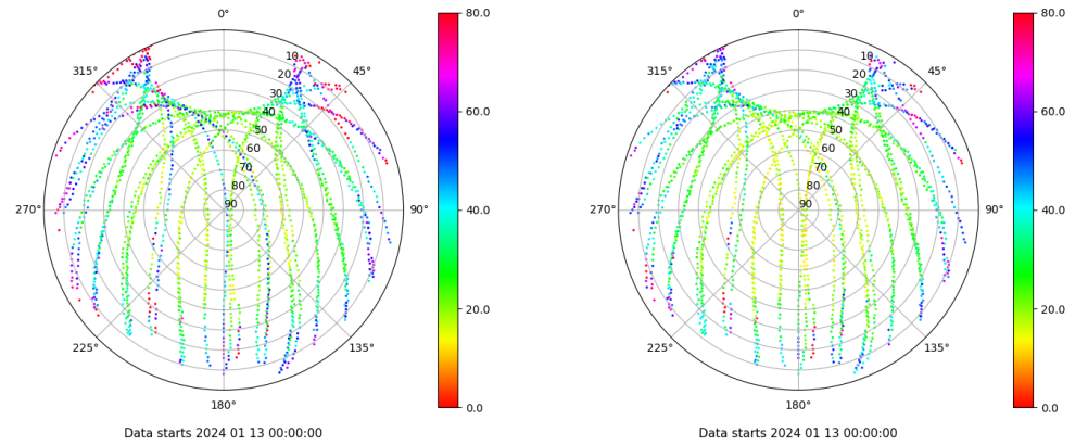
Skyplot for station ULP2. Parameter M1C Data file ULP200ESP_R_2024013.xtr Skyplot for station ULP2. Parameter M2C Data file ULP200ESP_R_2024013.xtr
