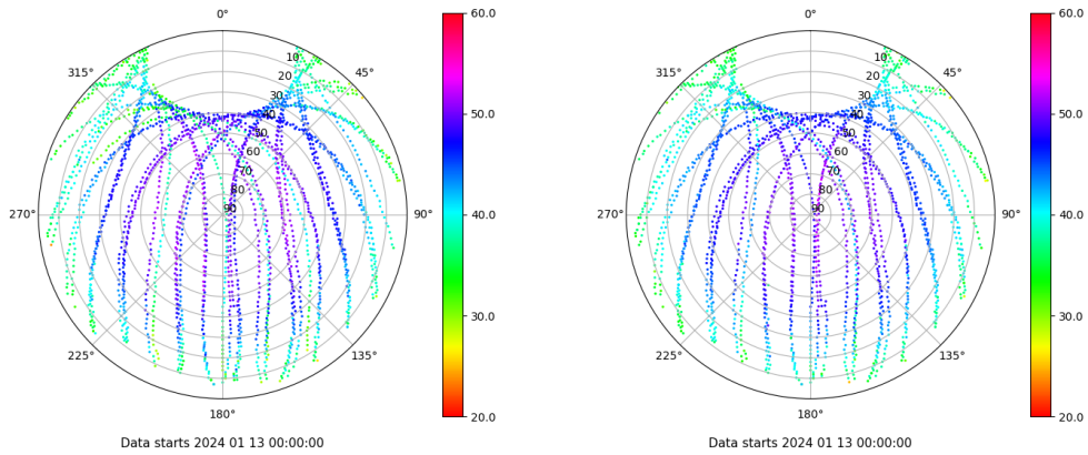
Skyplot for station ULP2. Signal to Noise S1C Data file ULP200ESP_R_2024013.xtr Skyplot for station ULP2. Signal to Noise S2C Data file ULP200ESP_R_2024013.xtr
