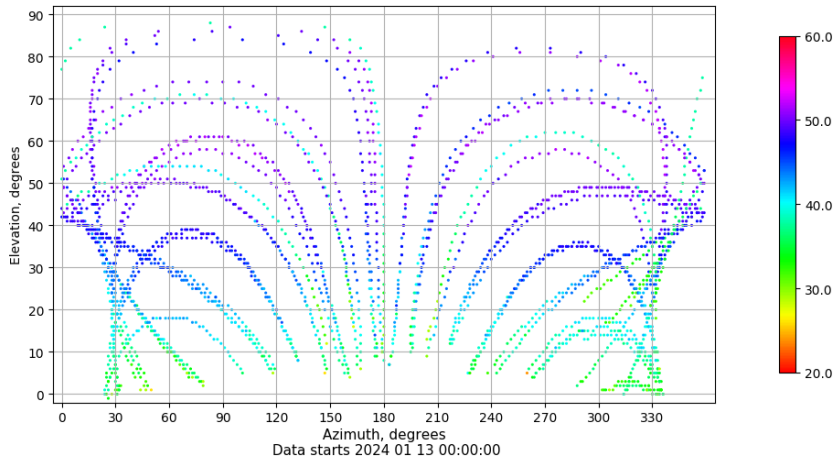
Azimuth-elevation plot for station ULP2. Signal to Noise S1C Data file ULP200ESP_R_2024013.xtr
