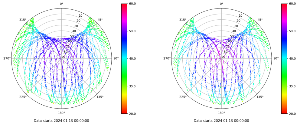
Skyplot for station ULP2. Signal to Noise S1C Data file ULP200ESP_R_2024013.xtr Skyplot for station ULP2. Signal to Noise S2X Data file ULP200ESP_R_2024013.xtr
