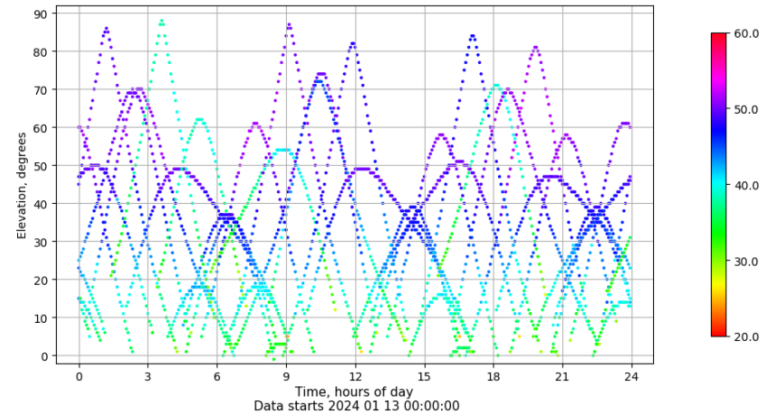
Time-elevation plot for station ULP2. Signal to Noise S1C Data file ULP200ESP_R_2024013.xtr
