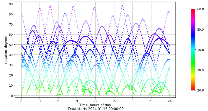
Time-elevation plot for station ULP2. Signal to Noise S1C Data file ULP200ESP_R_2024013.xtr
