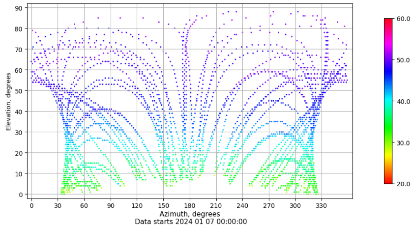
Azimuth-elevation plot for station ULP2. Signal to Noise S1C Data file ULP200ESP_R_2024007.xtr
