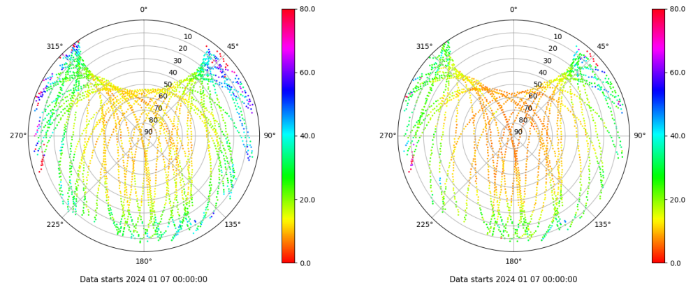
Skyplot for station ULP2. Parameter M1C Data file ULP200ESP_R_2024007.xtr Skyplot for station ULP2. Parameter M2X Data file ULP200ESP_R_2024007.xtr
