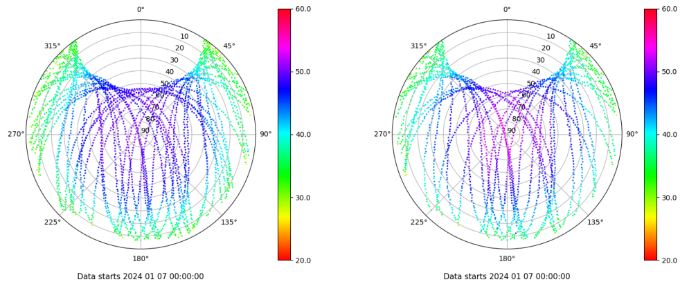
Skyplot for station ULP2. Signal to Noise S1C Data file ULP200ESP_R_2024007.xtr Skyplot for station ULP2. Signal to Noise S2X Data file ULP200ESP_R_2024007.xtr
