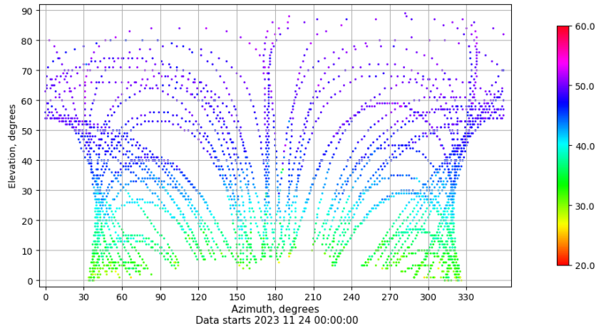
Azimuth-elevation plot for station ULP2. Signal to Noise S1C Data file ULP200ESP_R_2023328.xtr
