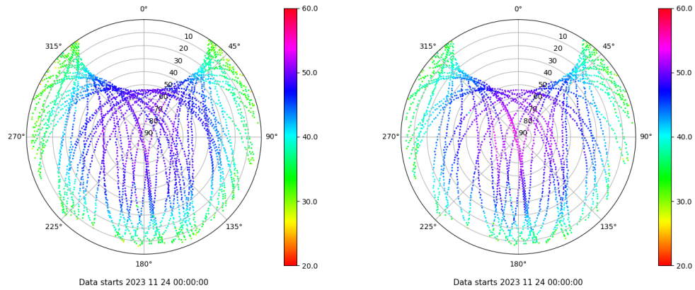
Skyplot for station ULP2. Signal to Noise S1C Data file ULP200ESP_R_2023328.xtr Skyplot for station ULP2. Signal to Noise S2X Data file ULP200ESP_R_2023328.xtr
