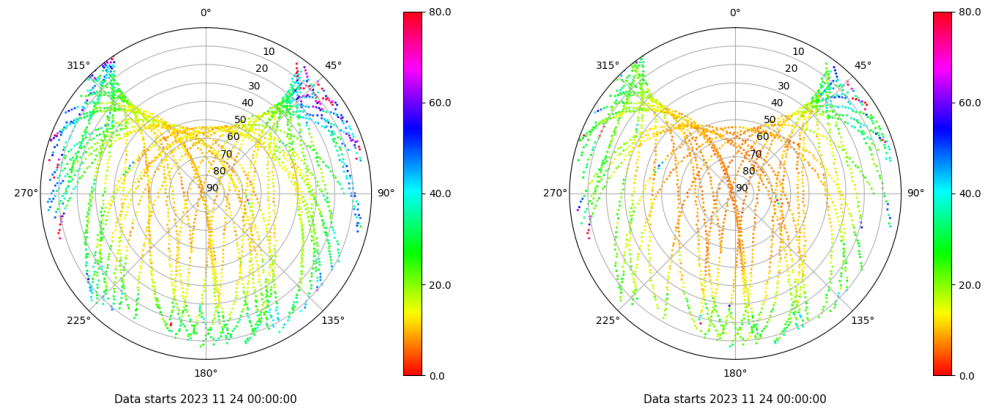
Skyplot for station ULP2. Parameter M1C Data file ULP200ESP_R_2023328.xtr Skyplot for station ULP2. Parameter M2X Data file ULP200ESP_R_2023328.xtr
