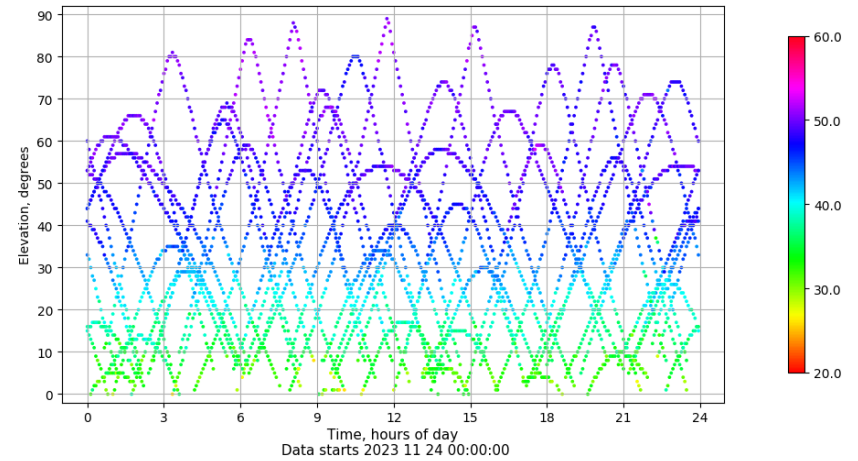
Time-elevation plot for station ULP2. Signal to Noise S1C Data file ULP200ESP_R_2023328.xtr
