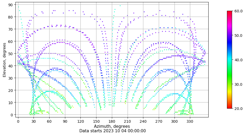
Azimuth-elevation plot for station ULP2. Signal to Noise S1C Data file ULP200ESP_R_2023277.xtr
