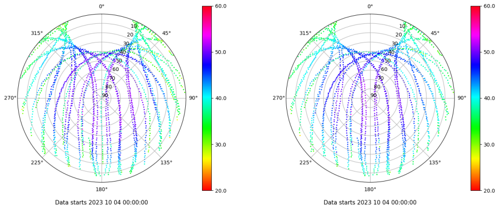
Skyplot for station ULP2. Signal to Noise S1C Data file ULP200ESP_R_2023277.xtr Skyplot for station ULP2. Signal to Noise S2C Data file ULP200ESP_R_2023277.xtr
