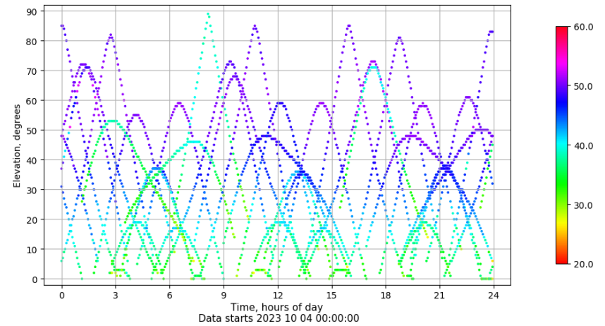
Time-elevation plot for station ULP2. Signal to Noise S1C Data file ULP200ESP_R_2023277.xtr
