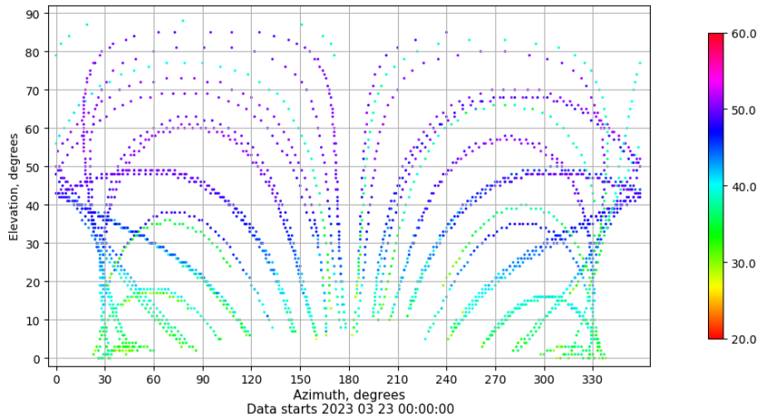
Azimuth-elevation plot for station ULP2. Signal to Noise S1C Data file ULP200ESP_R_2023082.xtr
