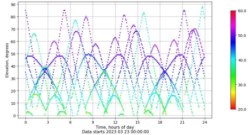
Time-elevation plot for station ULP2. Signal to Noise S1C Data file ULP200ESP_R_2023082.xtr
