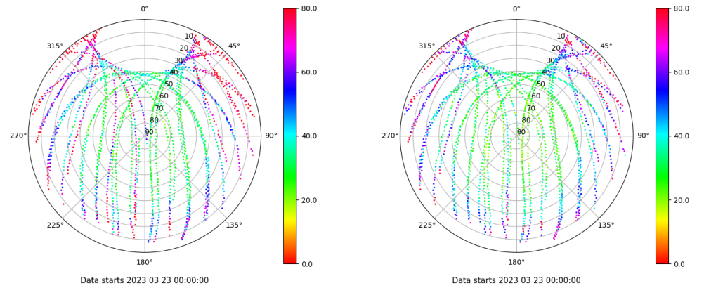
Skyplot for station ULP2. Parameter M1C Data file ULP200ESP_R_2023082.xtr Skyplot for station ULP2. Parameter M2C Data file ULP200ESP_R_2023082.xtr
