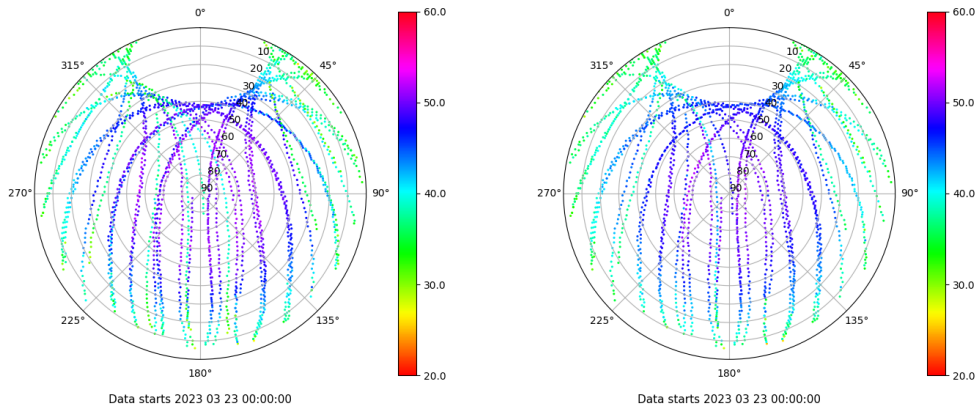
Skyplot for station ULP2. Signal to Noise S1C Data file ULP200ESP_R_2023082.xtr Skyplot for station ULP2. Signal to Noise S2C Data file ULP200ESP_R_2023082.xtr
