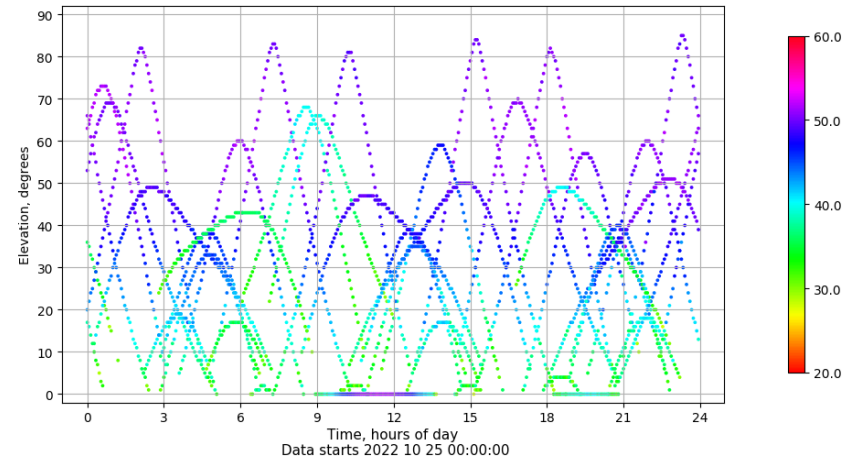
Time-elevation plot for station ULP2. Signal to Noise S1C Data file ULP200ESP_R_2022298.xtr
