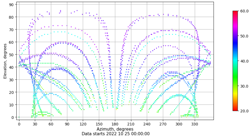
Azimuth-elevation plot for station ULP2. Signal to Noise S1C Data file ULP200ESP_R_2022298.xtr
