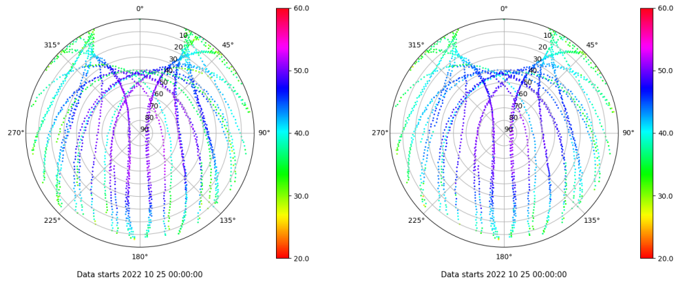
Skyplot for station ULP2. Signal to Noise S1C Data file ULP200ESP_R_2022298.xtr Skyplot for station ULP2. Signal to Noise S2C Data file ULP200ESP_R_2022298.xtr
