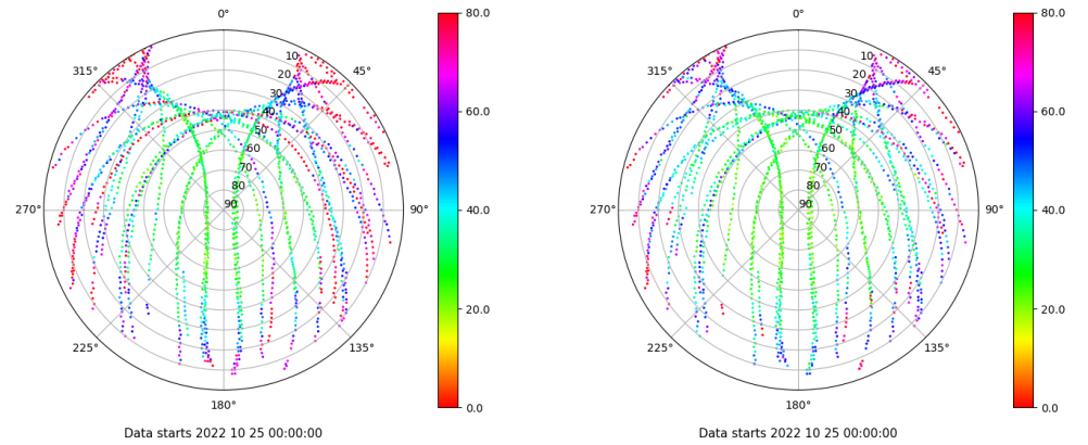
Skyplot for station ULP2. Parameter M1C Data file ULP200ESP_R_2022298.xtr Skyplot for station ULP2. Parameter M2C Data file ULP200ESP_R_2022298.xtr
