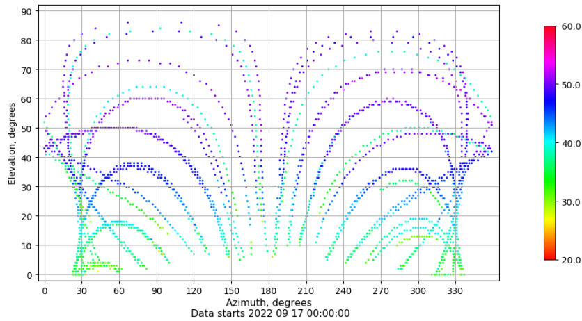
Azimuth-elevation plot for station ULP2. Signal to Noise S1C Data file ULP200ESP_R_2022260.xtr
