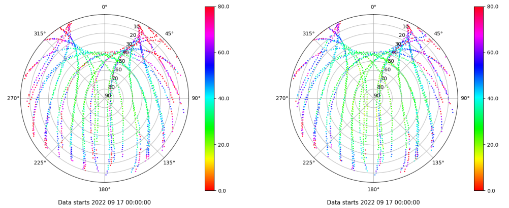
Skyplot for station ULP2. Parameter M1C Data file ULP200ESP_R_2022260.xtr Skyplot for station ULP2. Parameter M2C Data file ULP200ESP_R_2022260.xtr
