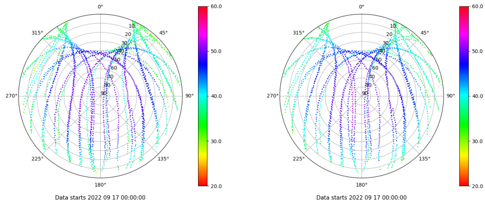
Skyplot for station ULP2. Signal to Noise S1C Data file ULP200ESP_R_2022260.xtr Skyplot for station ULP2. Signal to Noise S2C Data file ULP200ESP_R_2022260.xtr
