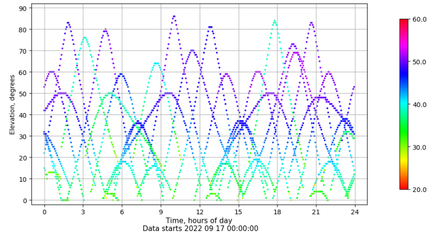
Time-elevation plot for station ULP2. Signal to Noise S1C Data file ULP200ESP_R_2022260.xtr
