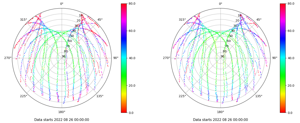
Skyplot for station ULP2. Parameter M1C Data file ULP200ESP_R_2022238.xtr Skyplot for station ULP2. Parameter M2C Data file ULP200ESP_R_2022238.xtr
