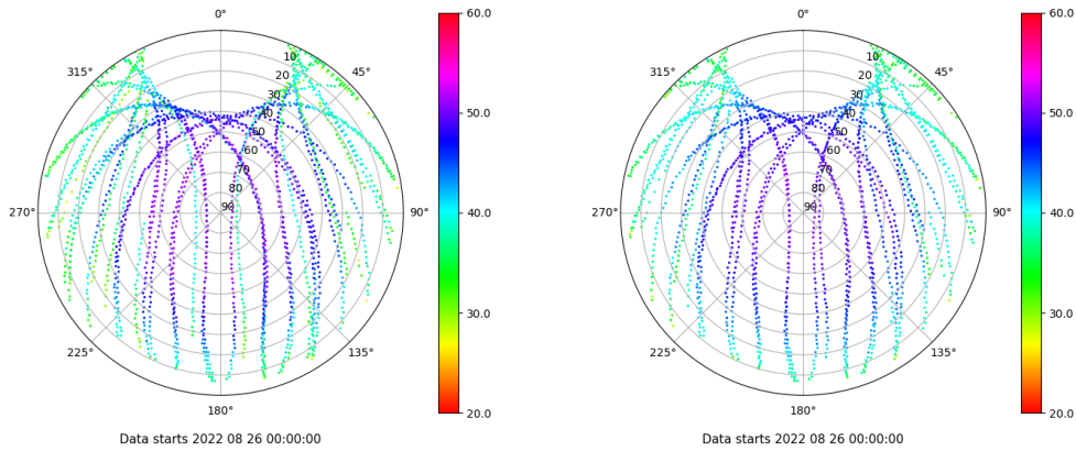
Skyplot for station ULP2. Signal to Noise S1C Data file ULP200ESP_R_2022238.xtr Skyplot for station ULP2. Signal to Noise S2C Data file ULP200ESP_R_2022238.xtr
