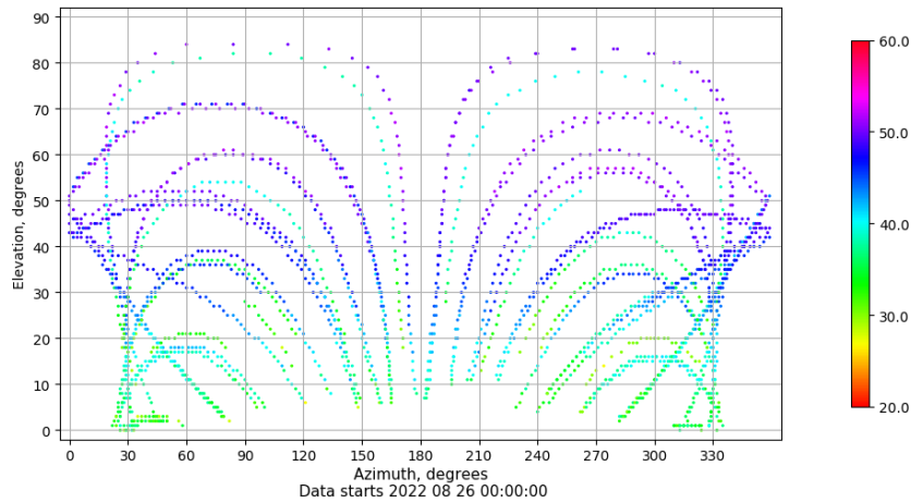
Azimuth-elevation plot for station ULP2. Signal to Noise S1C Data file ULP200ESP_R_2022238.xtr
