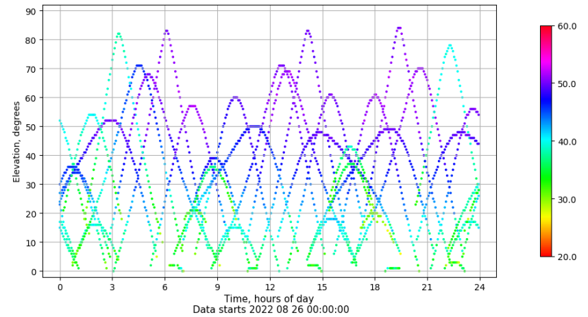
Time-elevation plot for station ULP2. Signal to Noise S1C Data file ULP200ESP_R_2022238.xtr
