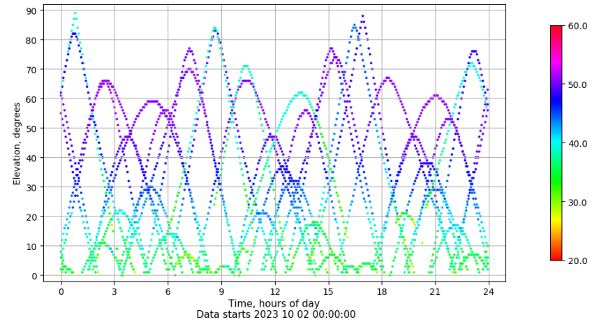
Time-elevation plot for station TUD1. Signal to Noise S1C Data file TUD100ESP_R_2023275.xtr
