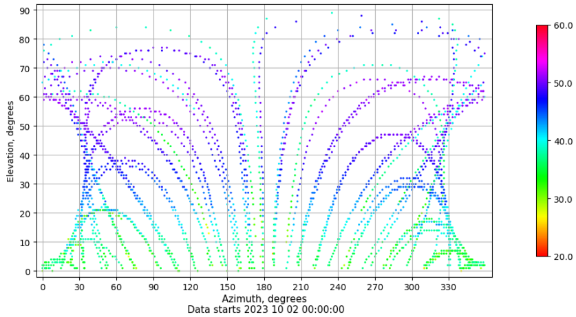
Azimuth-elevation plot for station TUD1. Signal to Noise S1C Data file TUD100ESP_R_2023275.xtr
