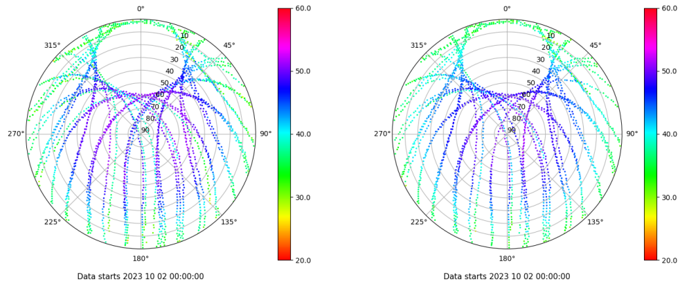
Skyplot for station TUD1. Signal to Noise S1C Data file TUD100ESP_R_2023275.xtr Skyplot for station TUD1. Signal to Noise S2C Data file TUD100ESP_R_2023275.xtr
