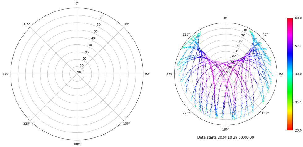
Skyplot for station TRAU. Signal to Noise S1C Data file TRAU00ESP_R_2024303.xtr Skyplot for station TRAU. Signal to Noise S2S Data file TRAU00ESP_R_2024303.xtr
