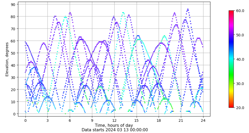
Time-elevation plot for station TRAU. Signal to Noise S1C Data file TRAU00ESP_R_2024073.xtr
