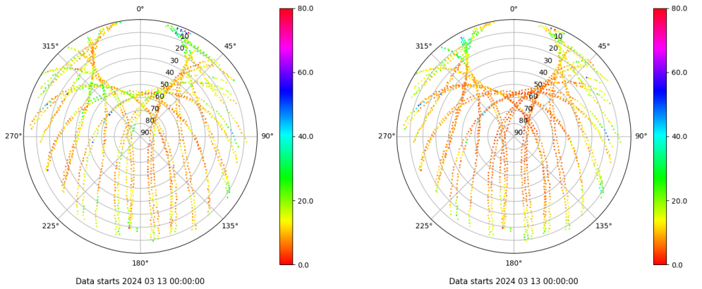
Skyplot for station TRAU. Parameter M1C Data file TRAU00ESP_R_2024073.xtr Skyplot for station TRAU. Parameter M2P Data file TRAU00ESP_R_2024073.xtr
