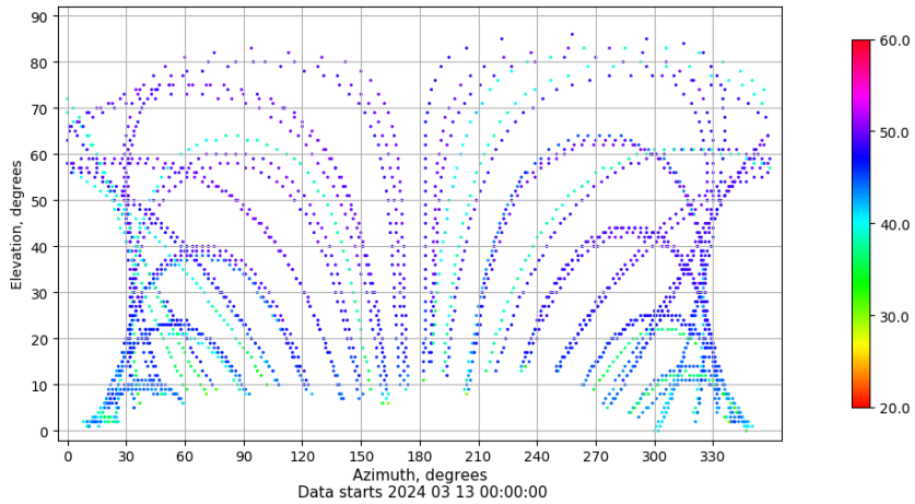
Azimuth-elevation plot for station TRAU. Signal to Noise S1C Data file TRAU00ESP_R_2024073.xtr
