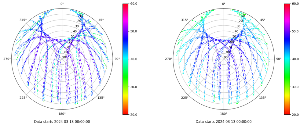
Skyplot for station TRAU. Signal to Noise S1C Data file TRAU00ESP_R_2024073.xtr Skyplot for station TRAU. Signal to Noise S2P Data file TRAU00ESP_R_2024073.xtr
