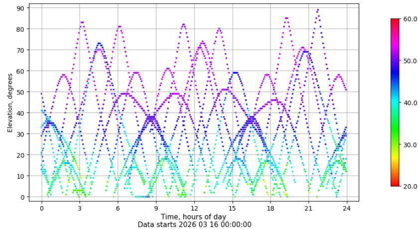
Time-elevation plot for station TN03. Signal to Noise S1C Data file TN0300ESP_R_2026075.xtr
