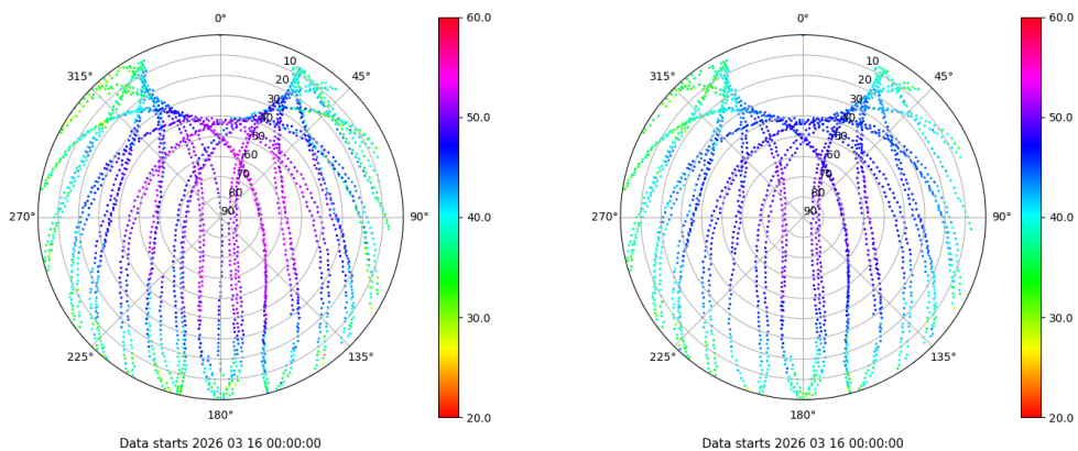
Skyplot for station TN03. Signal to Noise S1C Data file TN0300ESP_R_2026075.xtr Skyplot for station TN03. Signal to Noise S2C Data file TN0300ESP_R_2026075.xtr
