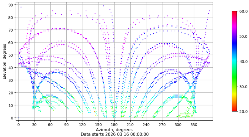
Azimuth-elevation plot for station TN03. Signal to Noise S1C Data file TN0300ESP_R_2026075.xtr
