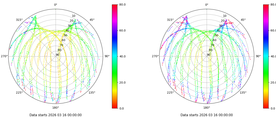
Skyplot for station TN03. Parameter M1C Data file TN0300ESP_R_2026075.xtr Skyplot for station TN03. Parameter M2C Data file TN0300ESP_R_2026075.xtr
