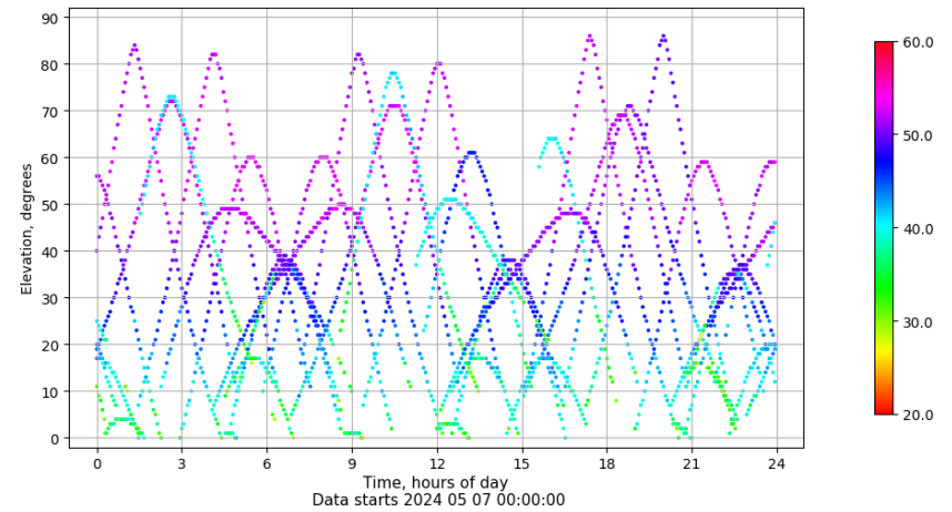
Time-elevation plot for station TN02. Signal to Noise S1C Data file TN0200ESP_R_2024128.xtr
