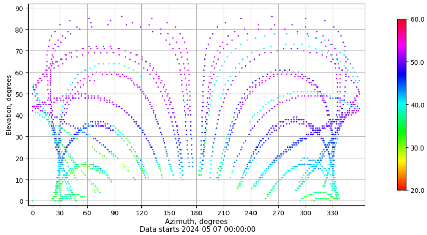
Azimuth-elevation plot for station TN02. Signal to Noise S1C Data file TN0200ESP_R_2024128.xtr
