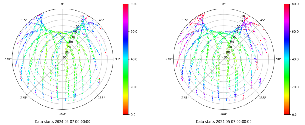
Skyplot for station TN02. Parameter M1C Data file TN0200ESP_R_2024128.xtr Skyplot for station TN02. Parameter M2C Data file TN0200ESP_R_2024128.xtr
