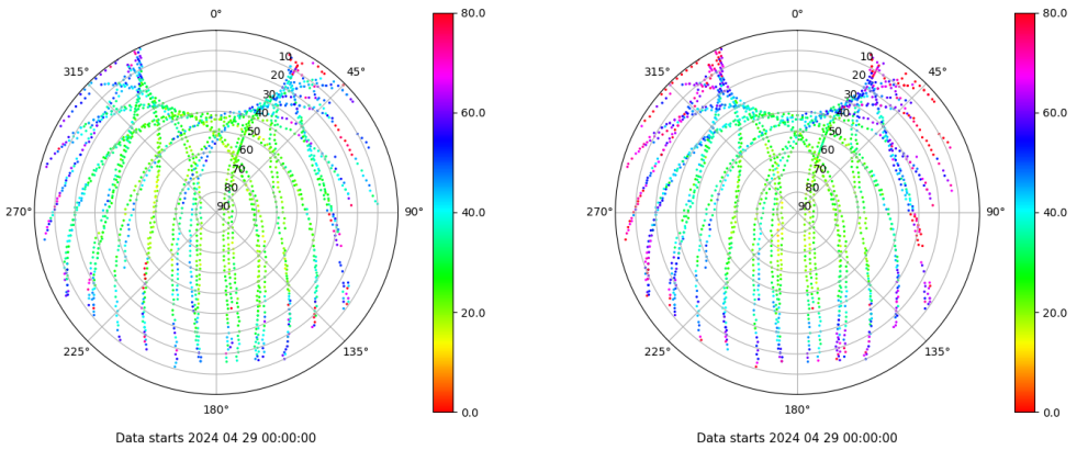
Skyplot for station TN02. Parameter M1C Data file TN0200ESP_R_2024120.xtr Skyplot for station TN02. Parameter M2C Data file TN0200ESP_R_2024120.xtr
