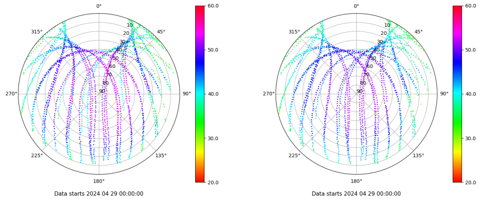
Skyplot for station TN02. Signal to Noise S1C Data file TN0200ESP_R_2024120.xtr Skyplot for station TN02. Signal to Noise S2C Data file TN0200ESP_R_2024120.xtr
