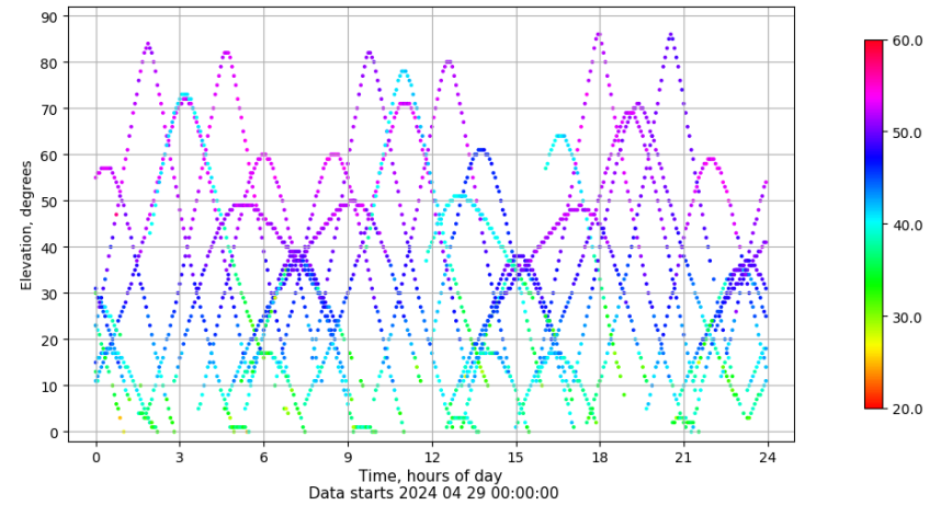
Time-elevation plot for station TN02. Signal to Noise S1C Data file TN0200ESP_R_2024120.xtr
