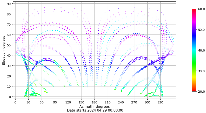
Azimuth-elevation plot for station TN02. Signal to Noise S1C Data file TN0200ESP_R_2024120.xtr
