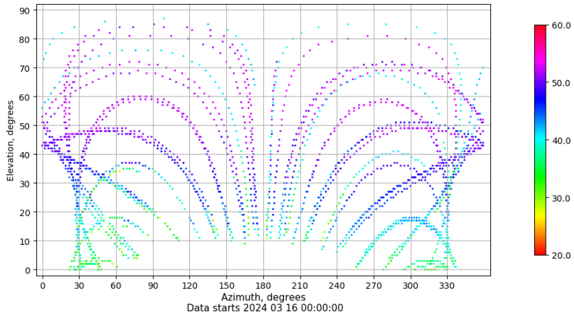
Azimuth-elevation plot for station TN02. Signal to Noise S1C Data file TN0200ESP_R_2024076.xtr
