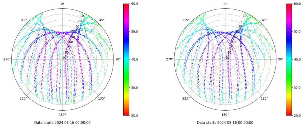
Skyplot for station TN02. Signal to Noise S1C Data file TN0200ESP_R_2024076.xtr Skyplot for station TN02. Signal to Noise S2C Data file TN0200ESP_R_2024076.xtr
