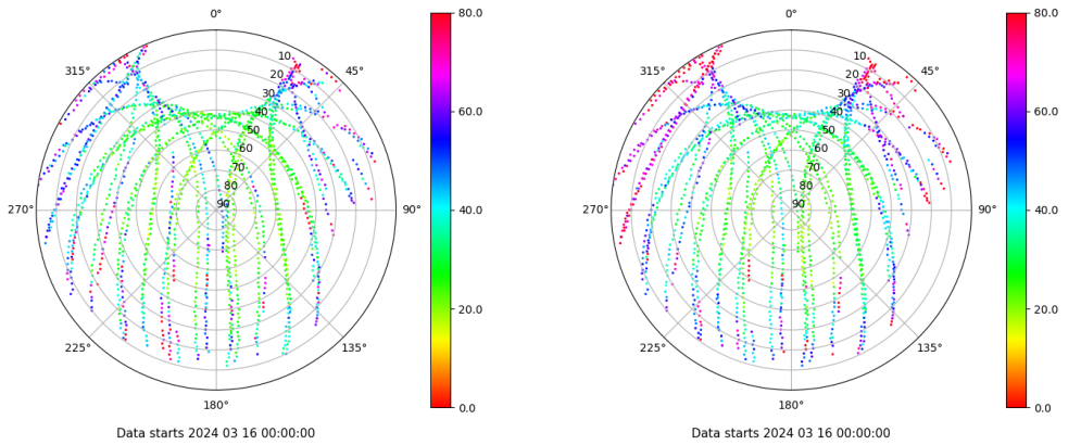
Skyplot for station TN02. Parameter M1C Data file TN0200ESP_R_2024076.xtr Skyplot for station TN02. Parameter M2C Data file TN0200ESP_R_2024076.xtr
