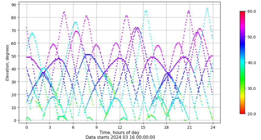
Time-elevation plot for station TN02. Signal to Noise S1C Data file TN0200ESP_R_2024076.xtr
