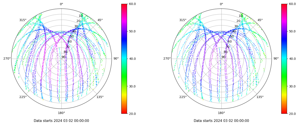
Skyplot for station TN02. Signal to Noise S1C Data file TN0200ESP_R_2024062.xtr Skyplot for station TN02. Signal to Noise S2C Data file TN0200ESP_R_2024062.xtr
