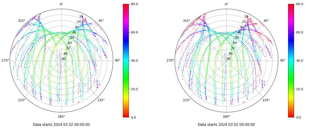
Skyplot for station TN02. Parameter M1C Data file TN0200ESP_R_2024062.xtr Skyplot for station TN02. Parameter M2C Data file TN0200ESP_R_2024062.xtr
