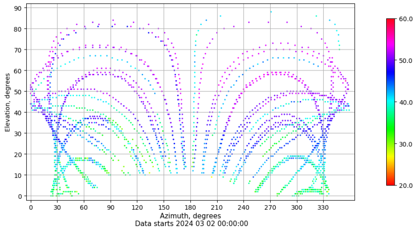
Azimuth-elevation plot for station TN02. Signal to Noise S1C Data file TN0200ESP_R_2024062.xtr
