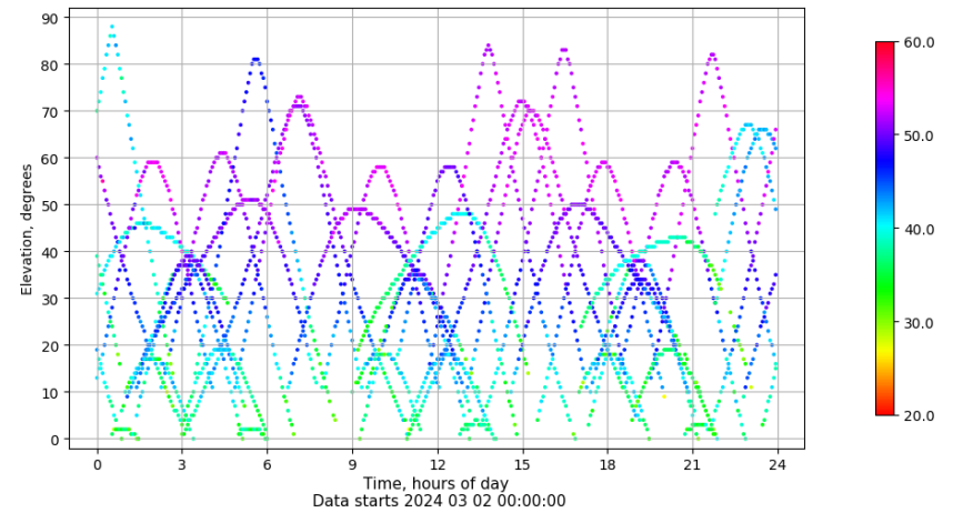
Time-elevation plot for station TN02. Signal to Noise S1C Data file TN0200ESP_R_2024062.xtr
