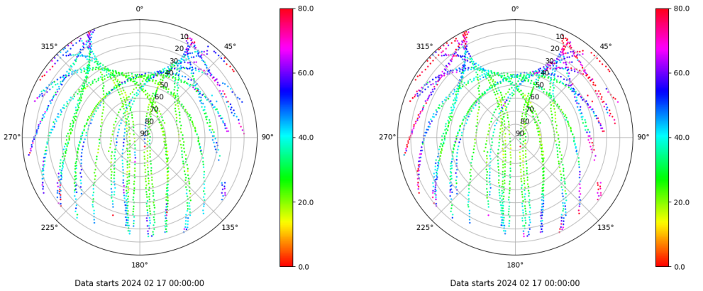
Skyplot for station TN02. Parameter M1C Data file TN0200ESP_R_2024048.xtr Skyplot for station TN02. Parameter M2C Data file TN0200ESP_R_2024048.xtr
