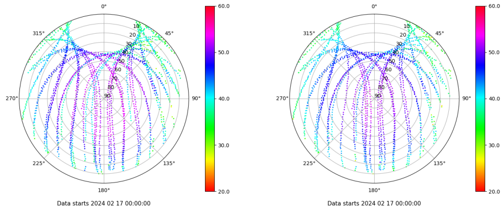
Skyplot for station TN02. Signal to Noise S1C Data file TN0200ESP_R_2024048.xtr Skyplot for station TN02. Signal to Noise S2C Data file TN0200ESP_R_2024048.xtr
