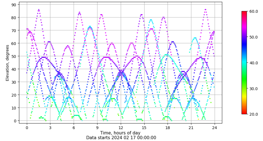
Time-elevation plot for station TN02. Signal to Noise S1C Data file TN0200ESP_R_2024048.xtr
