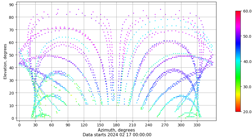
Azimuth-elevation plot for station TN02. Signal to Noise S1C Data file TN0200ESP_R_2024048.xtr
