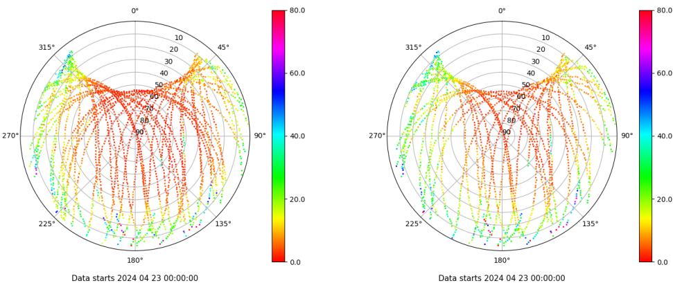
Skyplot for station TN01. Parameter M1C Data file TN0100ESP_R_2024114.xtr Skyplot for station TN01. Parameter M2S Data file TN0100ESP_R_2024114.xtr
