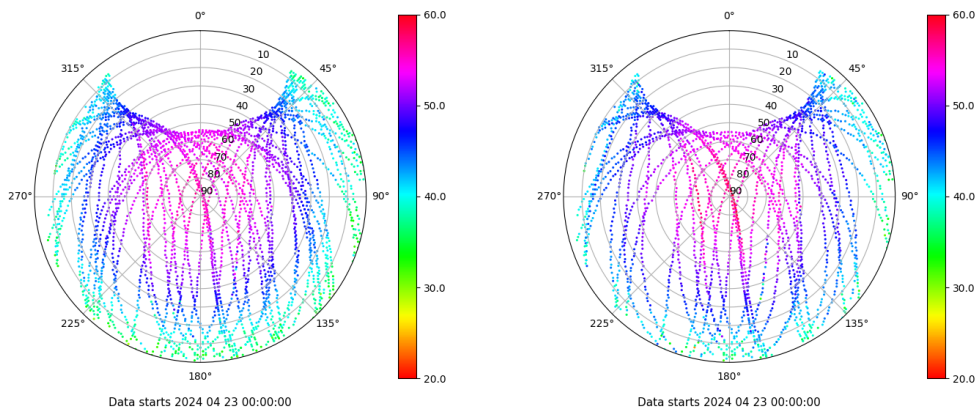
Skyplot for station TN01. Signal to Noise S1C Data file TN0100ESP_R_2024114.xtr Skyplot for station TN01. Signal to Noise S2S Data file TN0100ESP_R_2024114.xtr
