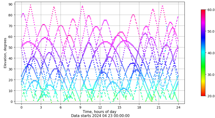
Time-elevation plot for station TN01. Signal to Noise S1C Data file TN0100ESP_R_2024114.xtr
