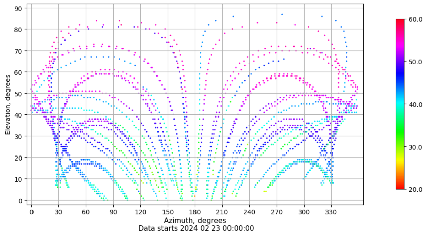
Azimuth-elevation plot for station TN01. Signal to Noise S1C Data file TN0100ESP_R_2024054.xtr
