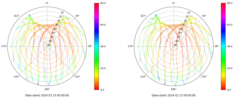
Skyplot for station TN01. Parameter M1C Data file TN0100ESP_R_2024054.xtr Skyplot for station TN01. Parameter M2C Data file TN0100ESP_R_2024054.xtr
