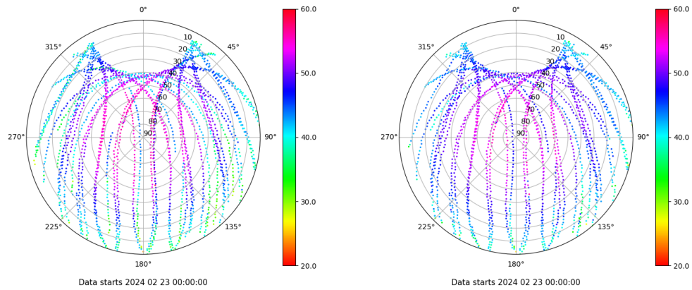
Skyplot for station TN01. Signal to Noise S1C Data file TN0100ESP_R_2024054.xtr Skyplot for station TN01. Signal to Noise S2C Data file TN0100ESP_R_2024054.xtr
