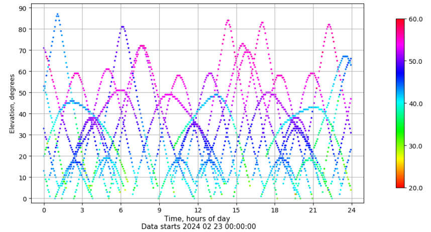
Time-elevation plot for station TN01. Signal to Noise S1C Data file TN0100ESP_R_2024054.xtr
