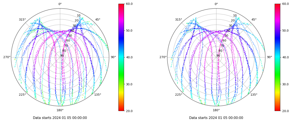
Skyplot for station TN01. Signal to Noise S1C Data file TN0100ESP_R_2024005.xtr Skyplot for station TN01. Signal to Noise S2C Data file TN0100ESP_R_2024005.xtr
