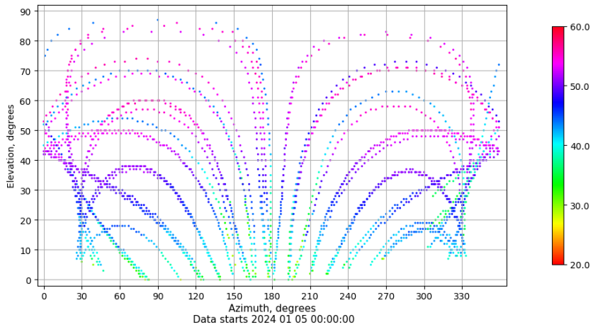
Azimuth-elevation plot for station TN01. Signal to Noise S1C Data file TN0100ESP_R_2024005.xtr
