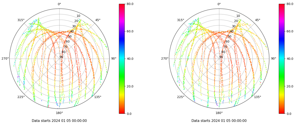
Skyplot for station TN01. Parameter M1C Data file TN0100ESP_R_2024005.xtr Skyplot for station TN01. Parameter M2C Data file TN0100ESP_R_2024005.xtr
