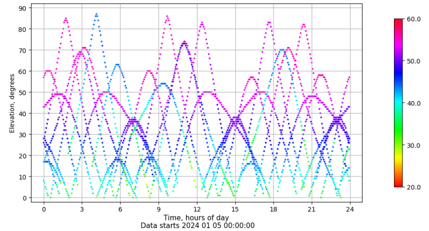
Time-elevation plot for station TN01. Signal to Noise S1C Data file TN0100ESP_R_2024005.xtr
