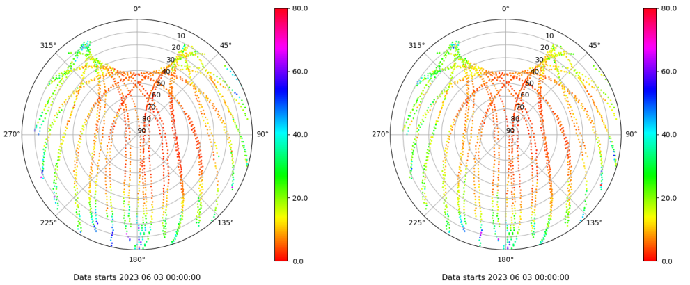
Skyplot for station TN01. Parameter M1C Data file TN0100ESP_R_2023154.xtr Skyplot for station TN01. Parameter M2C Data file TN0100ESP_R_2023154.xtr
