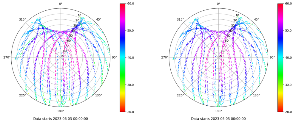
Skyplot for station TN01. Signal to Noise S1C Data file TN0100ESP_R_2023154.xtr Skyplot for station TN01. Signal to Noise S2C Data file TN0100ESP_R_2023154.xtr
