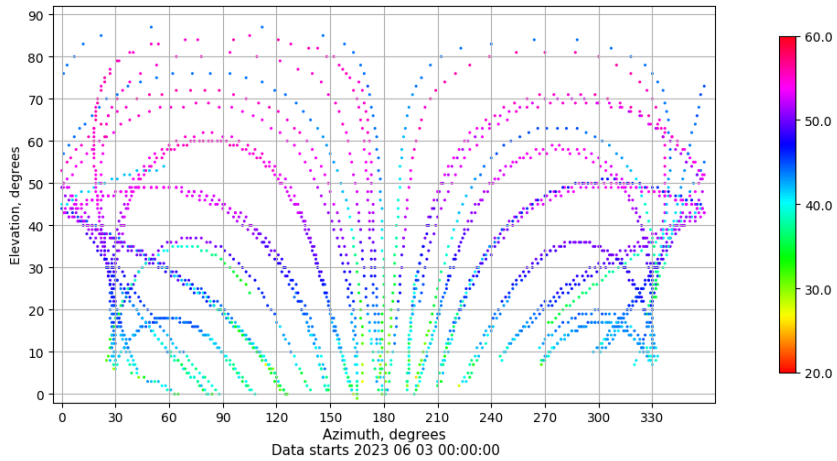
Azimuth-elevation plot for station TN01. Signal to Noise S1C Data file TN0100ESP_R_2023154.xtr
