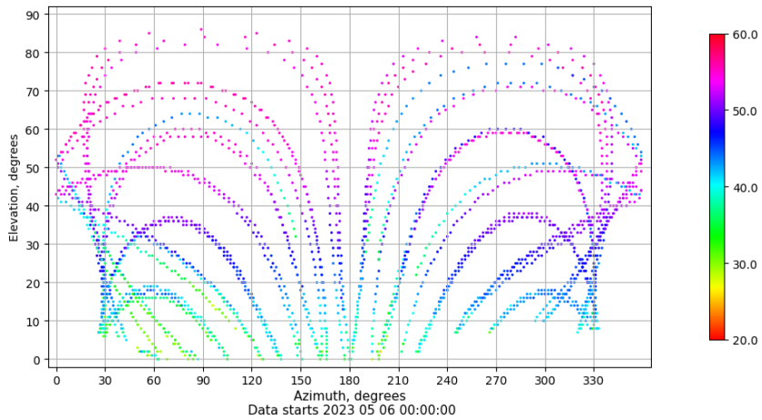
Azimuth-elevation plot for station TN01. Signal to Noise S1C Data file TN0100ESP_R_2023126.xtr
