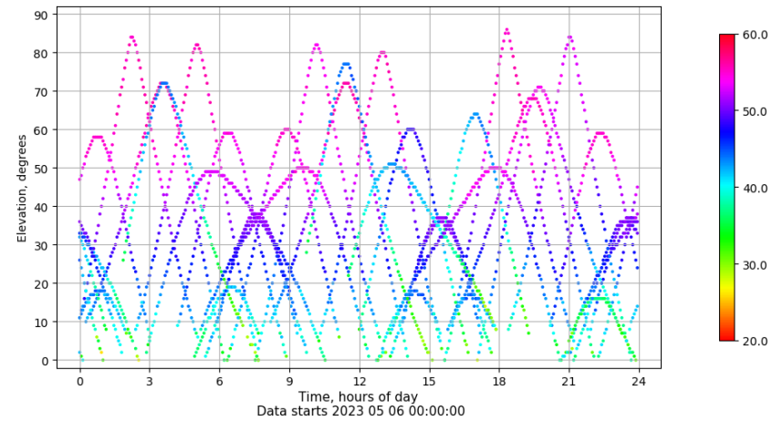
Time-elevation plot for station TN01. Signal to Noise S1C Data file TN0100ESP_R_2023126.xtr
