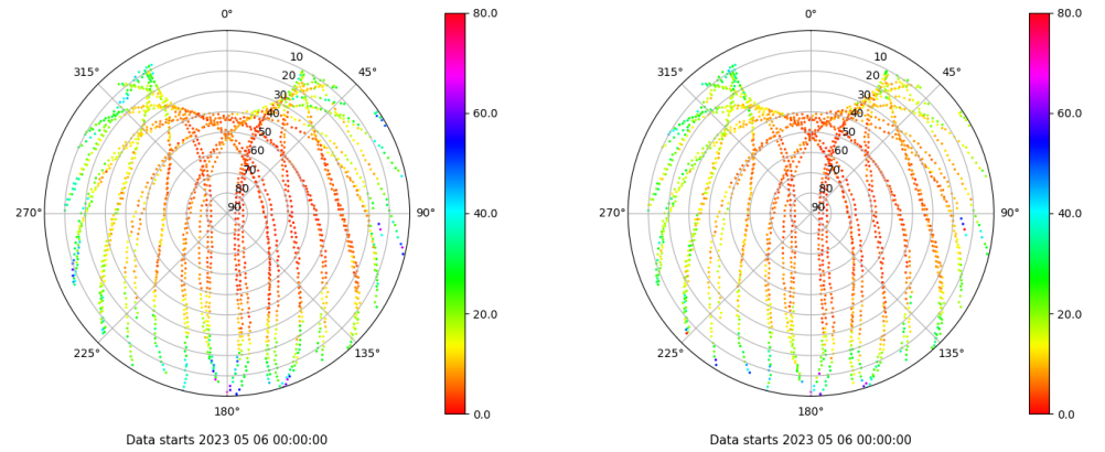
Skyplot for station TN01. Parameter M1C Data file TN0100ESP_R_2023126.xtr Skyplot for station TN01. Parameter M2C Data file TN0100ESP_R_2023126.xtr
