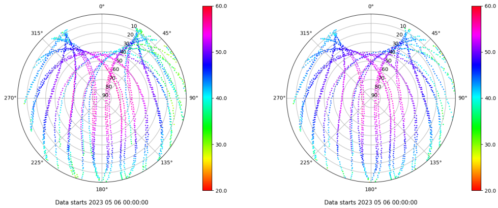
Skyplot for station TN01. Signal to Noise S1C Data file TN0100ESP_R_2023126.xtr Skyplot for station TN01. Signal to Noise S2C Data file TN0100ESP_R_2023126.xtr
