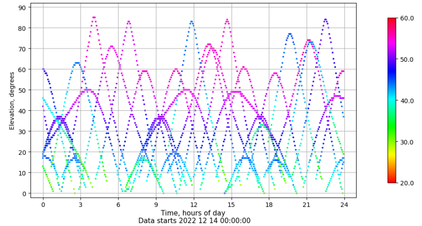
Time-elevation plot for station TN01. Signal to Noise S1C Data file TN0100ESP_R_2022348.xtr
