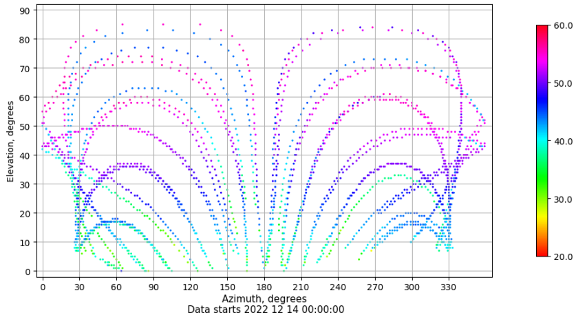
Azimuth-elevation plot for station TN01. Signal to Noise S1C Data file TN0100ESP_R_2022348.xtr
