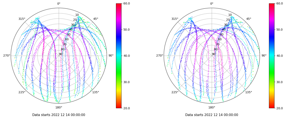
Skyplot for station TN01. Signal to Noise S1C Data file TN0100ESP_R_2022348.xtr Skyplot for station TN01. Signal to Noise S2C Data file TN0100ESP_R_2022348.xtr
