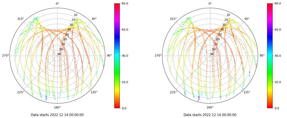
Skyplot for station TN01. Parameter M1C Data file TN0100ESP_R_2022348.xtr Skyplot for station TN01. Parameter M2C Data file TN0100ESP_R_2022348.xtr
