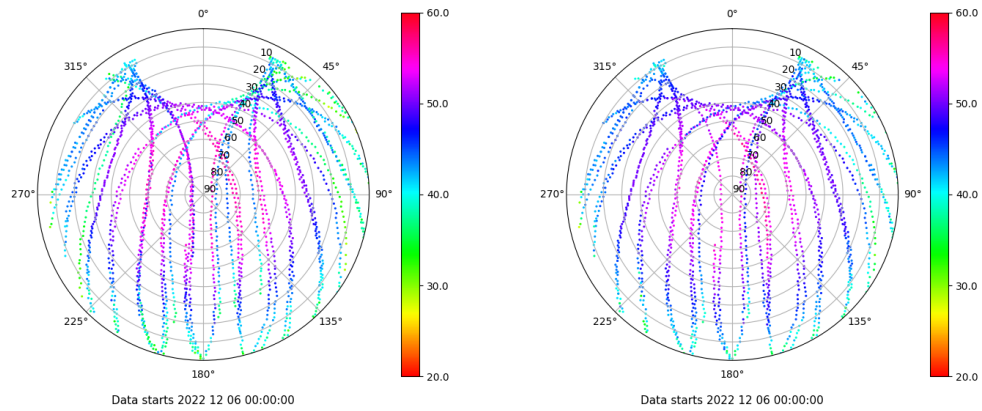
Skyplot for station TN01. Signal to Noise S1C Data file TN0100ESP_R_2022340.xtr Skyplot for station TN01. Signal to Noise S2C Data file TN0100ESP_R_2022340.xtr
