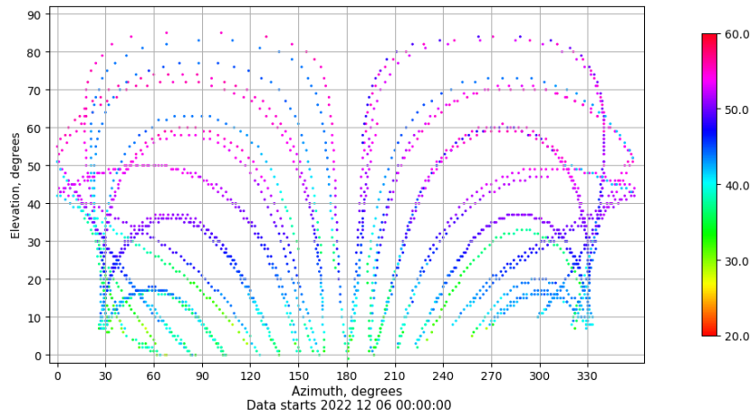
Azimuth-elevation plot for station TN01. Signal to Noise S1C Data file TN0100ESP_R_2022340.xtr
