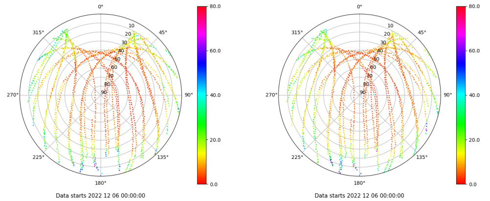
Skyplot for station TN01. Parameter M1C Data file TN0100ESP_R_2022340.xtr Skyplot for station TN01. Parameter M2C Data file TN0100ESP_R_2022340.xtr
