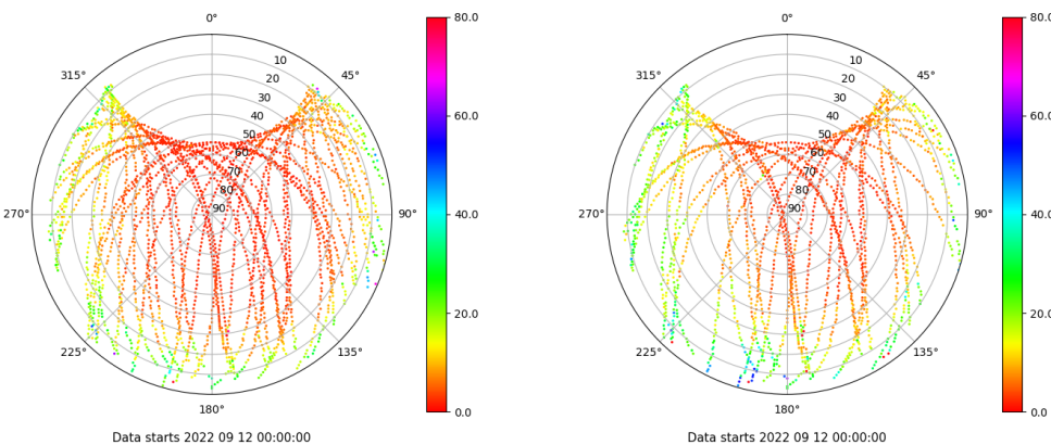
Skyplot for station TN01. Parameter M1C Data file TN0100ESP_R_2022255.xtr Skyplot for station TN01. Parameter M2S Data file TN0100ESP_R_2022255.xtr
