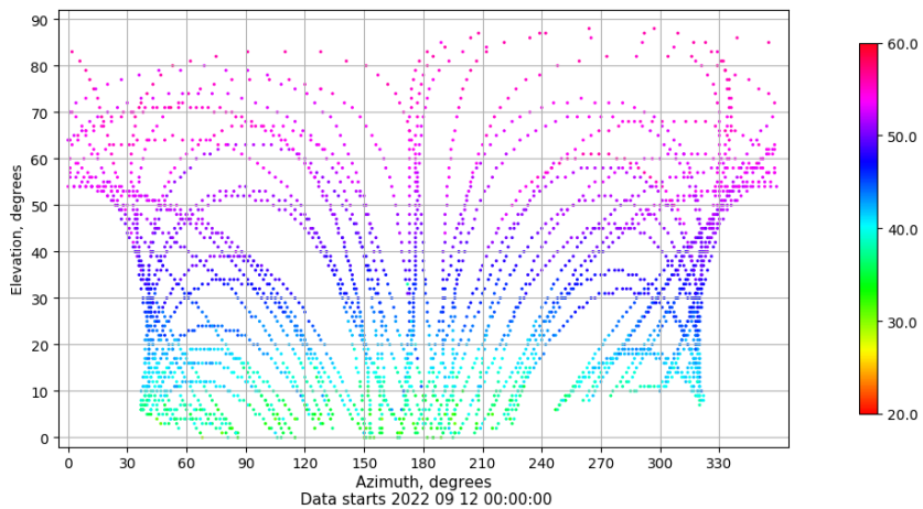
Azimuth-elevation plot for station TN01. Signal to Noise S1C Data file TN0100ESP_R_2022255.xtr
