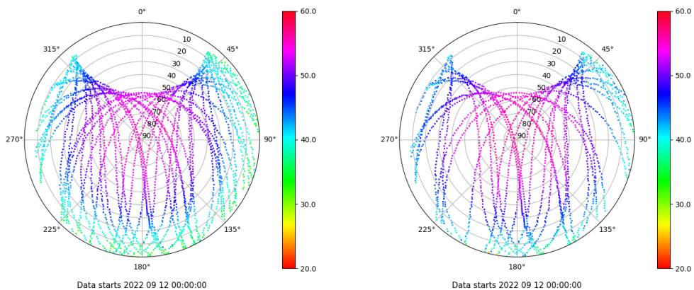
Skyplot for station TN01. Signal to Noise S1C Data file TN0100ESP_R_2022255.xtr Skyplot for station TN01. Signal to Noise S2S Data file TN0100ESP_R_2022255.xtr
