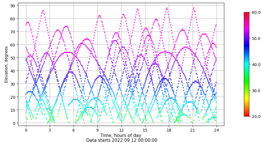
Time-elevation plot for station TN01. Signal to Noise S1C Data file TN0100ESP_R_2022255.xtr
