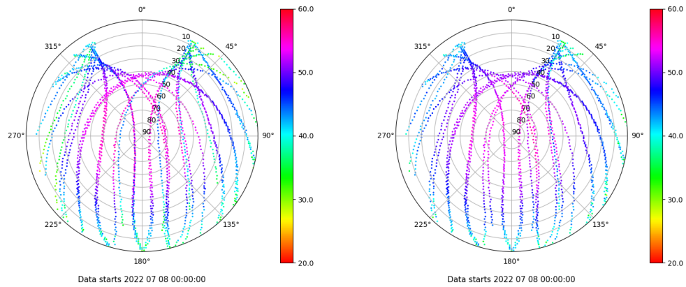
Skyplot for station TN01. Signal to Noise S1C Data file TN0100ESP_R_2022189.xtr Skyplot for station TN01. Signal to Noise S2C Data file TN0100ESP_R_2022189.xtr
