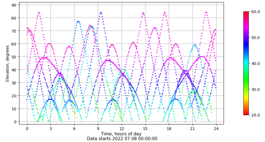
Time-elevation plot for station TN01. Signal to Noise S1C Data file TN0100ESP_R_2022189.xtr
