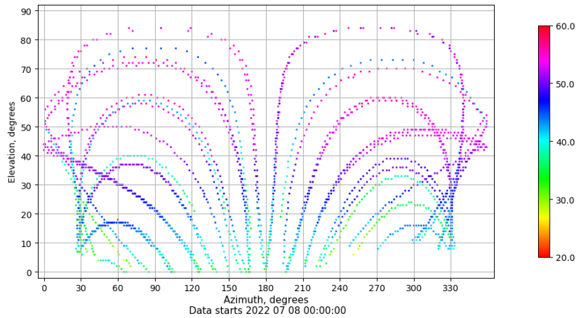
Azimuth-elevation plot for station TN01. Signal to Noise S1C Data file TN0100ESP_R_2022189.xtr
