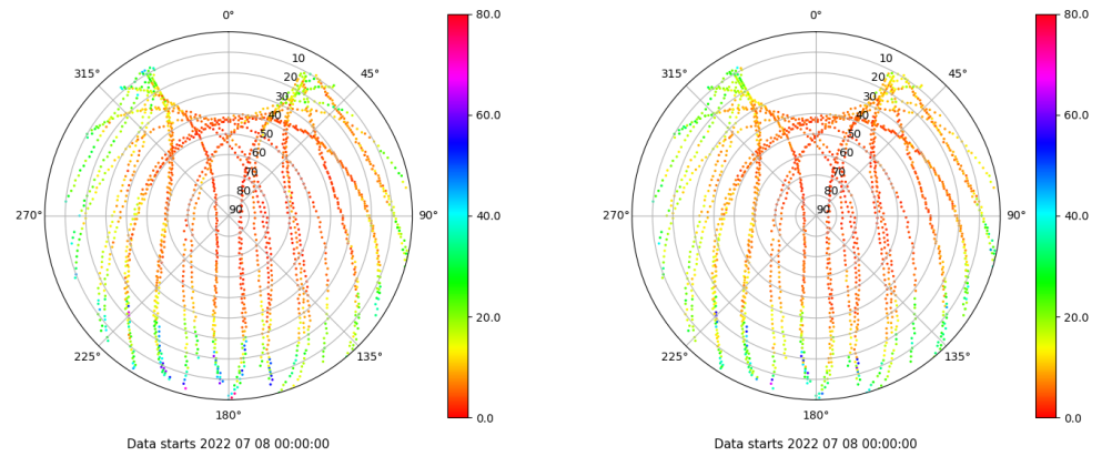
Skyplot for station TN01. Parameter M1C Data file TN0100ESP_R_2022189.xtr Skyplot for station TN01. Parameter M2C Data file TN0100ESP_R_2022189.xtr
