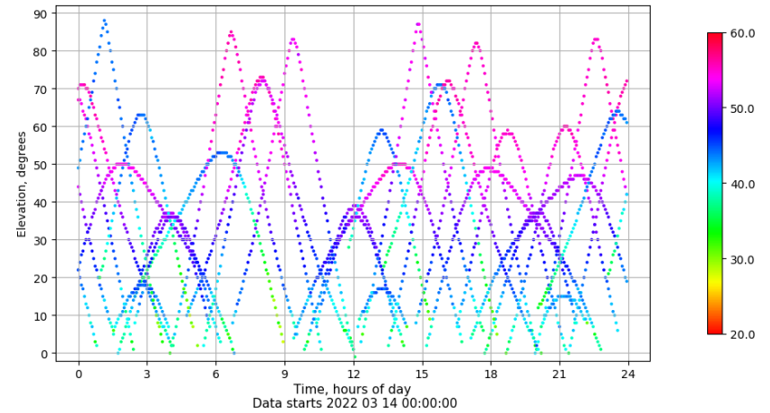
Time-elevation plot for station TN01. Signal to Noise S1C Data file TN0100ESP_R_2022073.xtr
