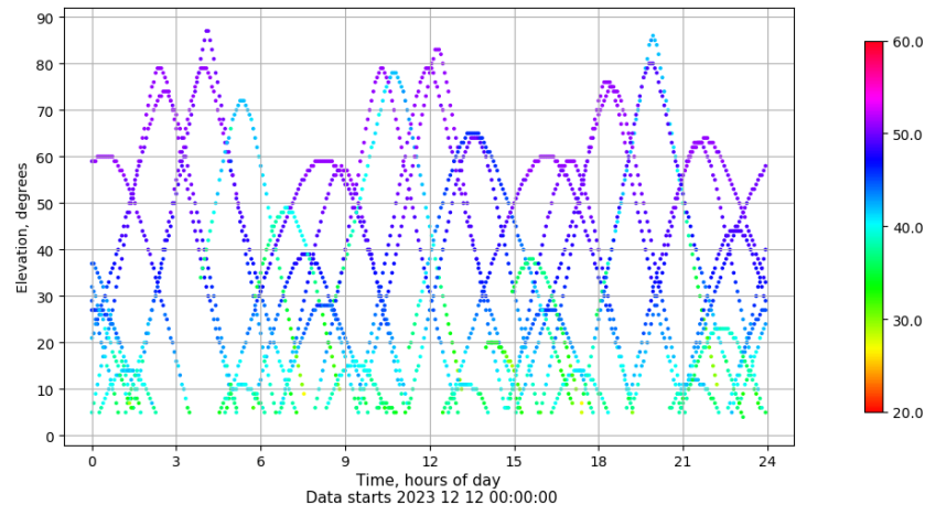
Time-elevation plot for station TARR. Signal to Noise S1C Data file TARR00ESP_R_2023346.xtr
