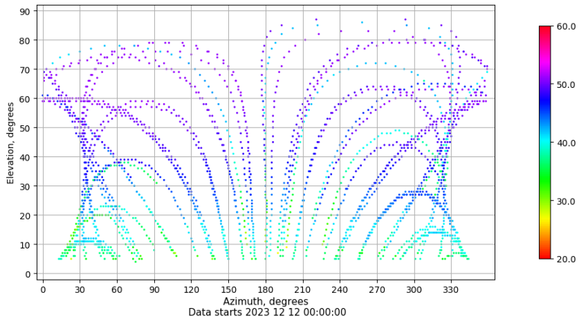
Azimuth-elevation plot for station TARR. Signal to Noise S1C Data file TARR00ESP_R_2023346.xtr
