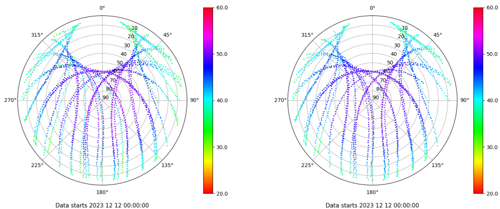
Skyplot for station TARR. Signal to Noise S1C Data file TARR00ESP_R_2023346.xtr Skyplot for station TARR. Signal to Noise S2P Data file TARR00ESP_R_2023346.xtr
