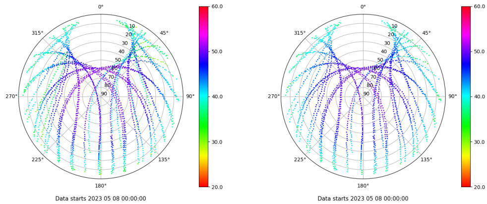
Skyplot for station TARR. Signal to Noise S1C Data file TARR00ESP_R_2023128.xtr Skyplot for station TARR. Signal to Noise S2P Data file TARR00ESP_R_2023128.xtr
