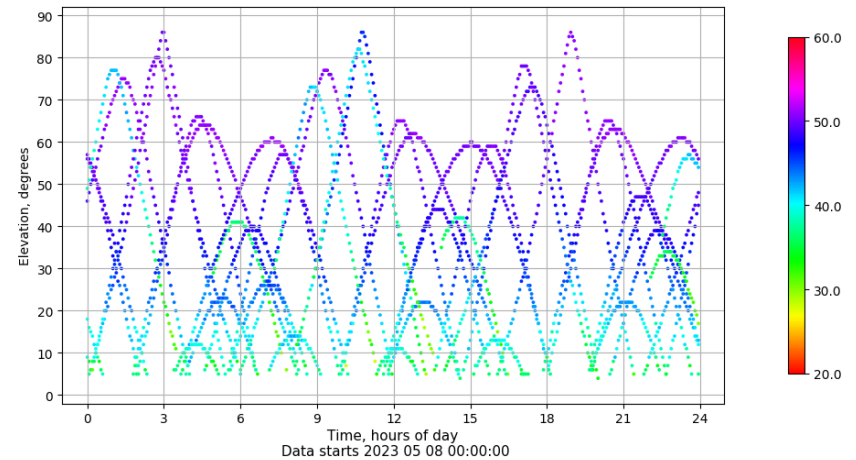
Time-elevation plot for station TARR. Signal to Noise S1C Data file TARR00ESP_R_2023128.xtr
