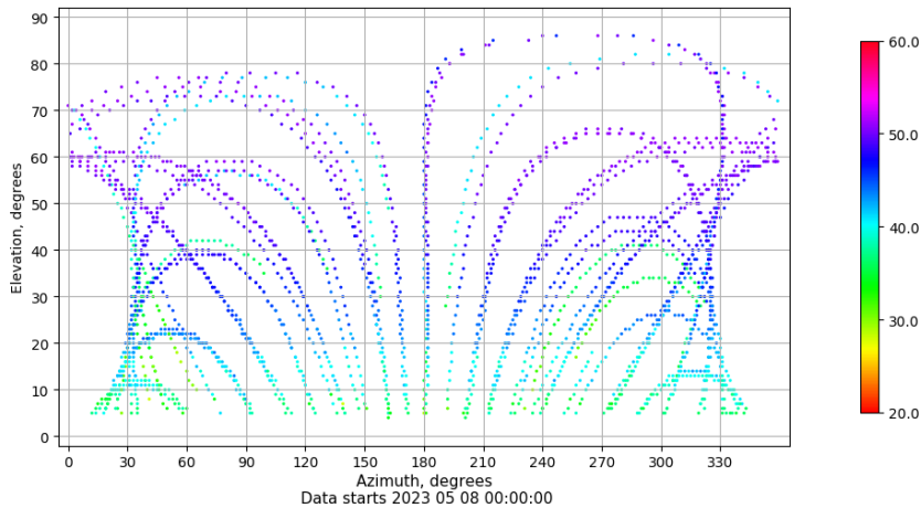
Azimuth-elevation plot for station TARR. Signal to Noise S1C Data file TARR00ESP_R_2023128.xtr
