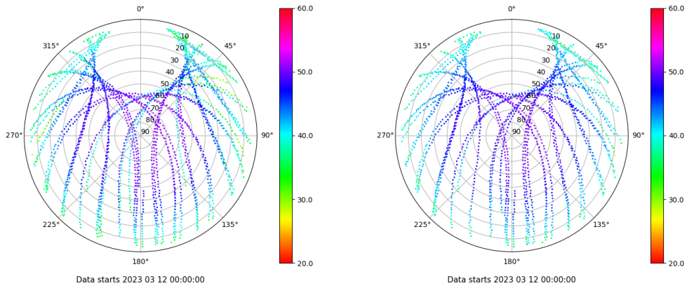
Skyplot for station TARR. Signal to Noise S1C Data file TARR00ESP_R_2023071.xtr Skyplot for station TARR. Signal to Noise S2P Data file TARR00ESP_R_2023071.xtr
