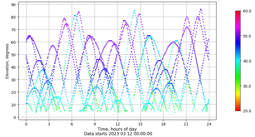
Time-elevation plot for station TARR. Signal to Noise S1C Data file TARR00ESP_R_2023071.xtr
