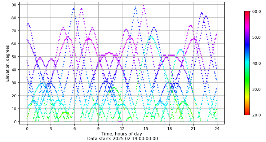
Time-elevation plot for station TAR2. Signal to Noise S1C Data file TAR200ESP_R_2025050.xtr
