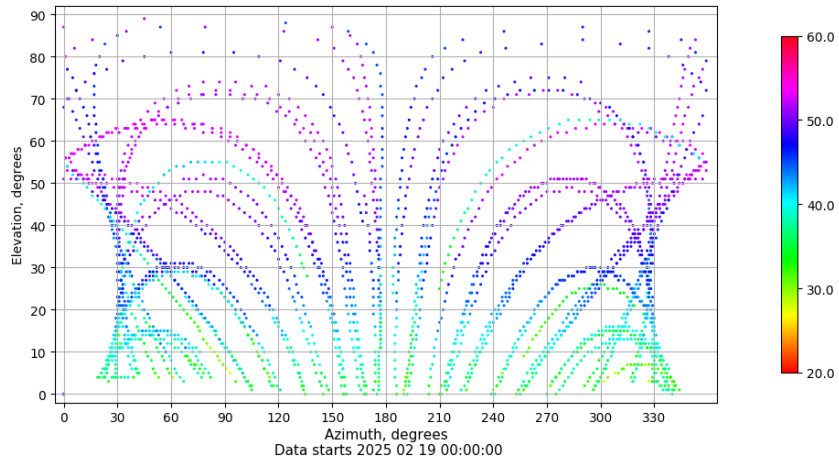
Azimuth-elevation plot for station TAR2. Signal to Noise S1C Data file TAR200ESP_R_2025050.xtr
