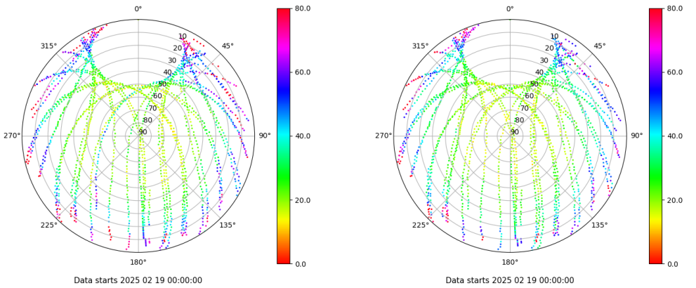
Skyplot for station TAR2. Parameter M1C Data file TAR200ESP_R_2025050.xtr Skyplot for station TAR2. Parameter M2C Data file TAR200ESP_R_2025050.xtr
