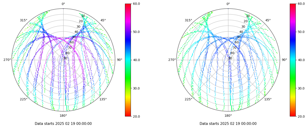
Skyplot for station TAR2. Signal to Noise S1C Data file TAR200ESP_R_2025050.xtr Skyplot for station TAR2. Signal to Noise S2C Data file TAR200ESP_R_2025050.xtr
